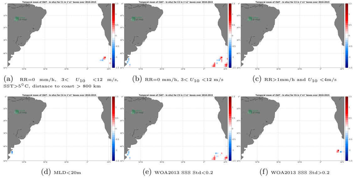
Figure 12: Temporal mean gridded over spatial boxes of size 1^\circ \times 1^\circ of \Delta SSS (SMOS-L3-CATDS-CPDC-V317-MONTHLY-25KM - Sea mammals) for 6 different subdatasets corresponding to: RR=0 mm/h, 3 < U_{10} < 12 m/s, SST > 5^\circ\text{C} , distance to coast > 800 km (a), RR=0 mm/h, 3 < U_{10} < 12 m/s (b), RR > 1 mm/h and U_{10} < 4 m/s (c), MLD < 20 m (d), WOA2013 SSS Std < 0.2 (e), WOA2013 SSS Std > 0.2 (f).
