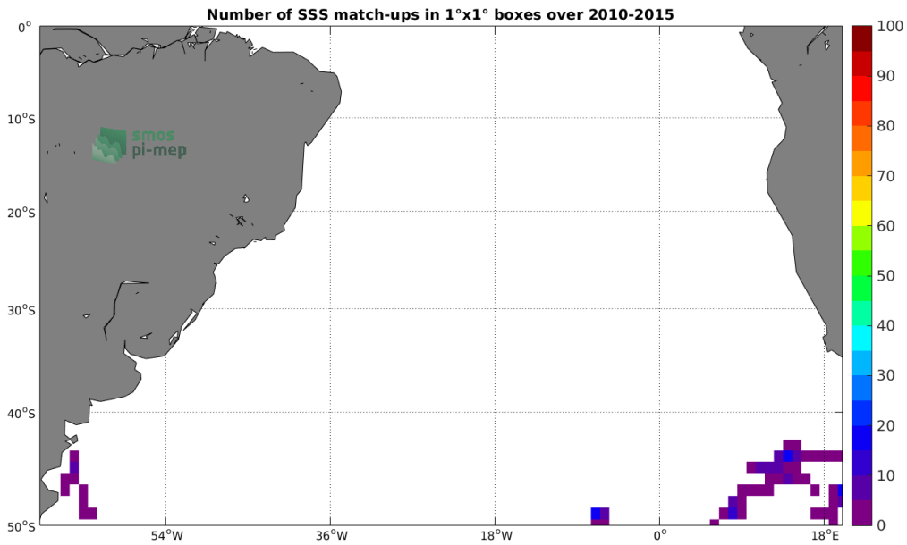
Figure 4: Number of SSS match-ups between Sea mammals SSS and the SMOS-L3-CATDS-CPDC-V317-MONTHLY-25KM SSS product for the South Atlantic Ocean Pi-MEP region over 1°x1° boxes and for the full satellite product period.
