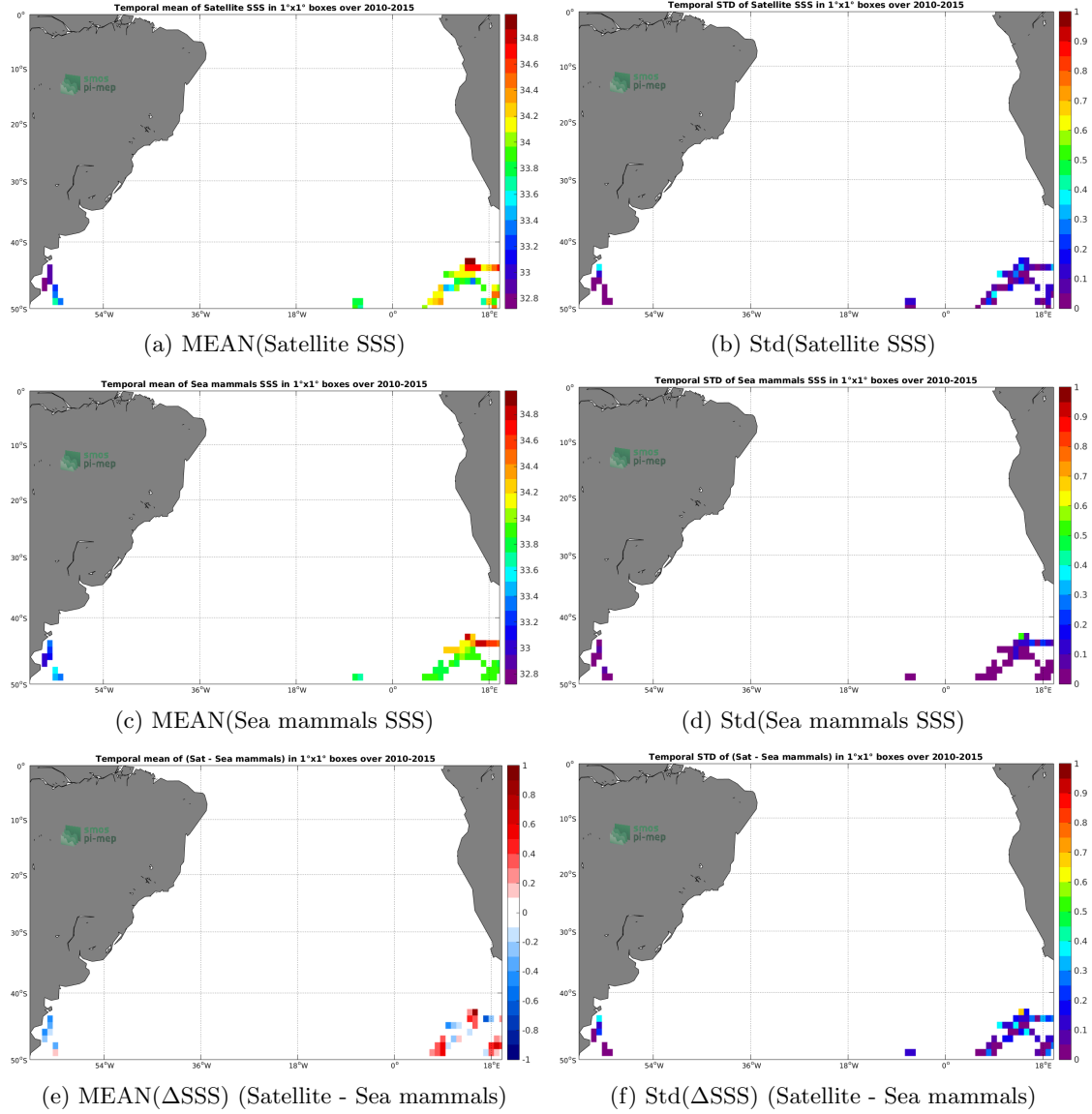
Figure 6: Temporal mean (left) and Std (right) of SSS from SMOS-L3-CATDS-CPDC-V317-MONTHLY-25KM (top), Sea mammals (middle), and of \Delta SSS (Satellite - Sea mammals). Only match-up pairs are used to generate these maps.
