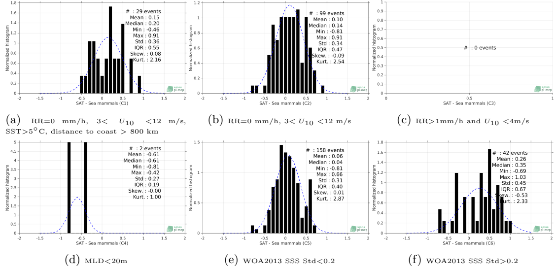
Figure 13: Normalized histogram of \Delta\text{SSS} (SMOS-L3-CATDS-CPDC-V317-MONTHLY-25KM - Sea mammals) for 6 different subdatasets corresponding to: RR=0 mm/h, 3 < U_{10} < 12 m/s, SST > 5^{\circ}\text{C} , distance to coast > 800 km (a), RR=0 mm/h, 3 < U_{10} < 12 m/s (b), RR > 1\text{mm/h} and U_{10} < 4\text{m/s} (c), MLD < 20\text{m} (d), WOA2013 SSS Std < 0.2 (e), WOA2013 SSS Std > 0.2 (f).
