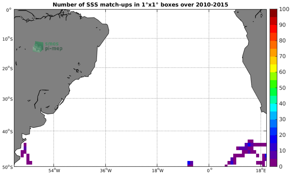
Figure 4: Number of SSS match-ups between Sea mammals SSS and the SMOS-L3-CATDS-CPDC-V317-MONTHLY-25KM SSS product for the South Atlantic Ocean Pi-MEP region over 1^\circ \times 1^\circ boxes and for the full satellite product period.
