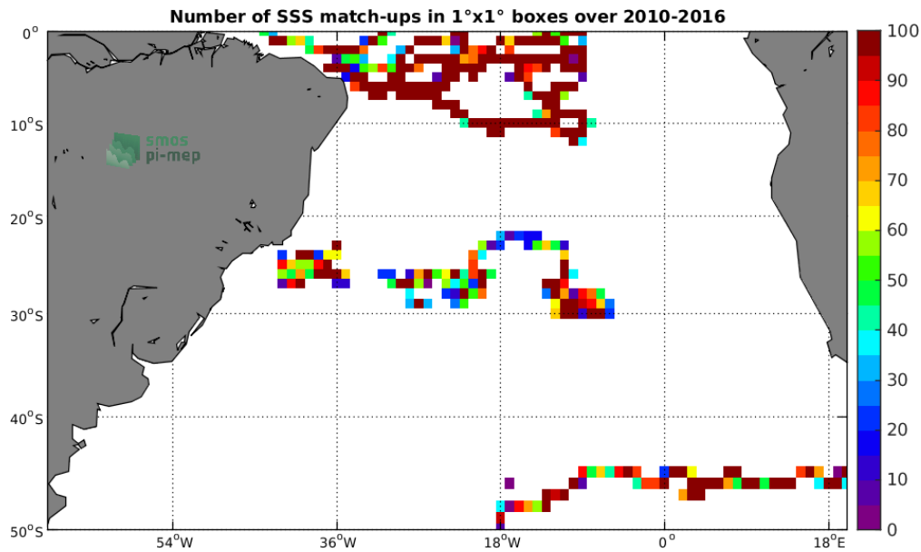
Figure 3: Number of SSS match-ups between Surface drifters SSS and the SMOS-L3-CATDS-CPDC-V317-MONTHLY-25KM SSS product for the South Atlantic Ocean Pi-MEP region over 1^\circ \times 1^\circ boxes and for the full satellite product period.
