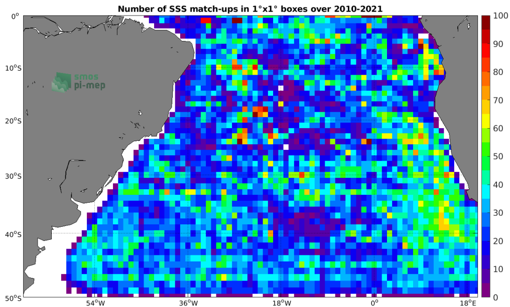
Figure 4: Number of SSS match-ups between Argo SSS and the SMOS SSS L3 v317 - Monthly - 25 km (CATDS-CPDC) SSS product for the South Atlantic Ocean Pi-MEP region over 1^\circ \times 1^\circ boxes and for the full satellite product period.
