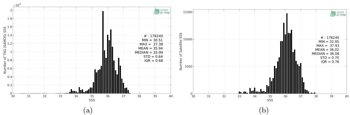
Figure 2: Histograms of SSS from TSG (SAMOS) (a) and SMOS SSS L3 v317 - 10 Days - 25 km (CATDS-CPDC) (b) considering all match-up pairs per bins of 0.1 over the South Atlantic Ocean Pi-MEP region and for the full satellite product period.
