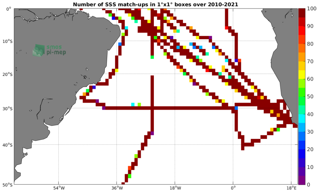
Figure 4: Number of SSS match-ups between TSG (SAMOS) SSS and the SMOS SSS L3 v317 - 10 Days - 25 km (CATDS-CPDC) SSS product for the South Atlantic Ocean Pi-MEP region over 1^\circ \times 1^\circ boxes and for the full satellite product period.
