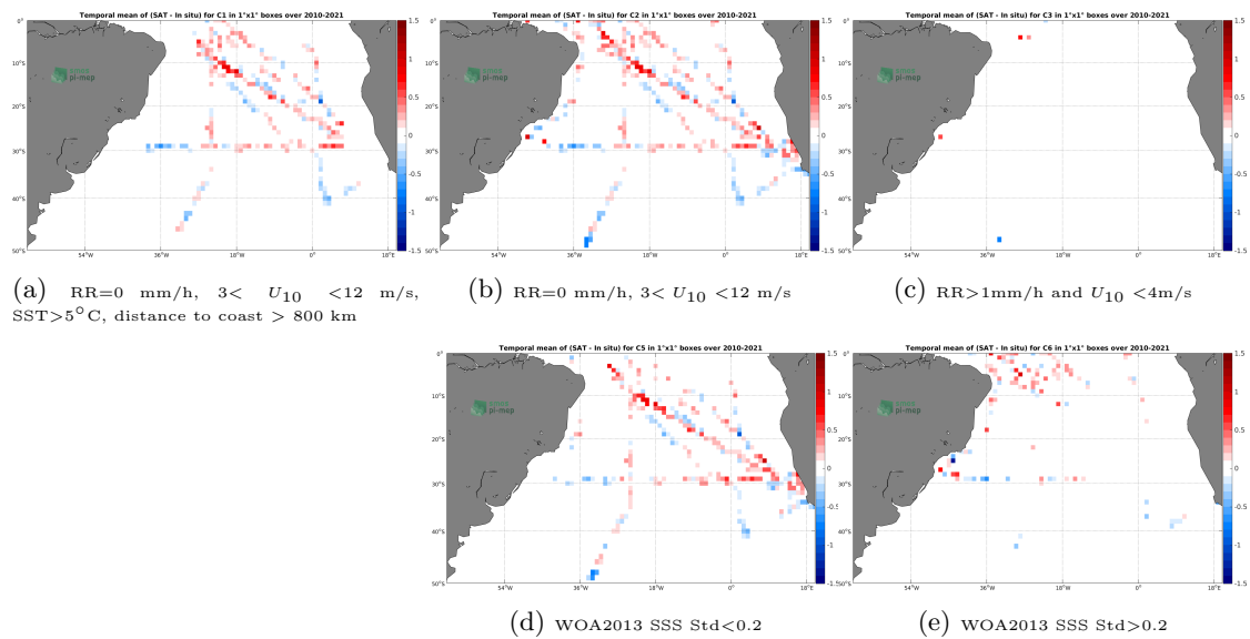
Figure 12: Temporal mean gridded over spatial boxes of size 1^\circ \times 1^\circ of \Delta SSS (SMOS SSS L3 v317 - 10 Days - 25 km (CATDS-CPDC) - TSG (SAMOS)) for 5 different subdatasets corresponding to: RR=0 mm/h, 3 < U_{10} < 12 m/s, SST > 5^\circ\text{C} , distance to coast > 800 km (a), RR=0 mm/h, 3 < U_{10} < 12 m/s (b), RR > 1 mm/h and U_{10} < 4 m/s (c), WOA2013 SSS Std < 0.2 (d), WOA2013 SSS Std > 0.2 (e).
