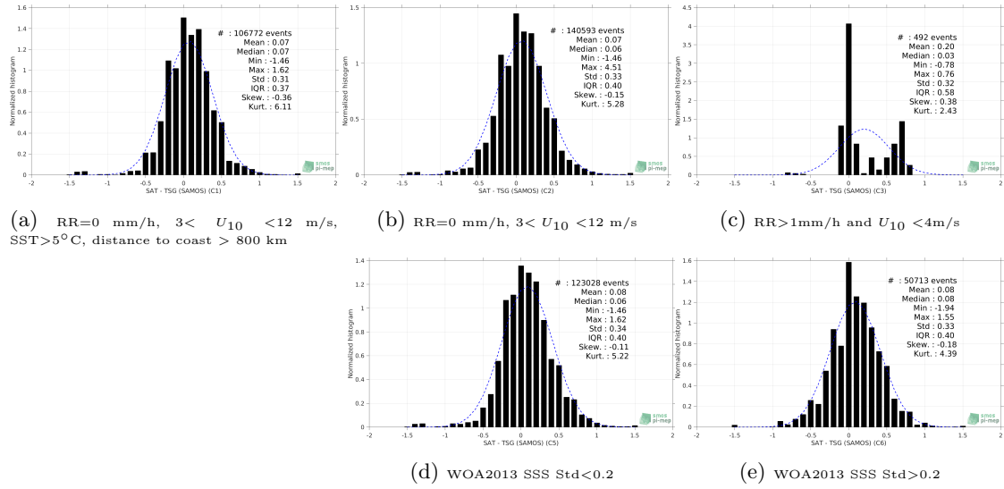
Figure 13: Normalized histogram of \Delta SSS (SMOS SSS L3 v317 - 10 Days - 25 km (CATDS-CPDC) - TSG (SAMOS)) for 5 different subdatasets corresponding to: RR=0 mm/h, 3 < U_{10} < 12 m/s, SST > 5°C, distance to coast > 800 km (a), RR=0 mm/h, 3 < U_{10} < 12 m/s (b), RR > 1mm/h and U_{10} < 4 m/s (c), WOA2013 SSS Std < 0.2 (d), WOA2013 SSS Std > 0.2 (e).
