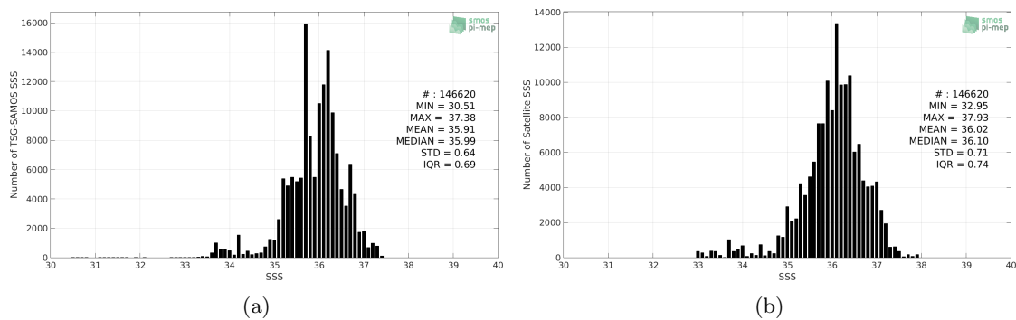
Figure 2: Histograms of SSS from TSG-SAMOS (a) and SMOS-L3-CATDS-CPDC-V317-10DAYS-25KM (b) considering all match-up pairs per bins of 0.1 over the South Atlantic Ocean Pi-MEP region and for the full satellite product period.
