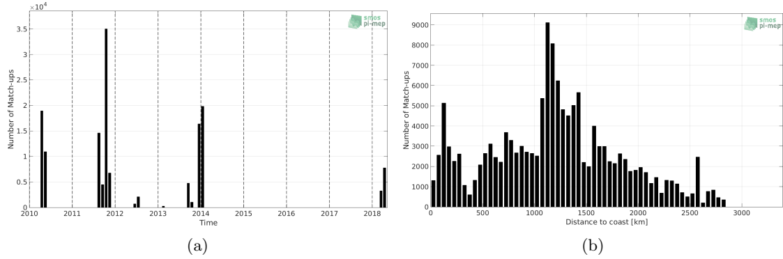
Figure 1: Number of match-ups between TSG-SAMOS and SMOS-L3-CATDS-CPDC-V317-10DAYS-25KM SSS as a function of time (a) and as function of the distance to coast (b) over the South Atlantic Ocean Pi-MEP region and for the full satellite product period.
