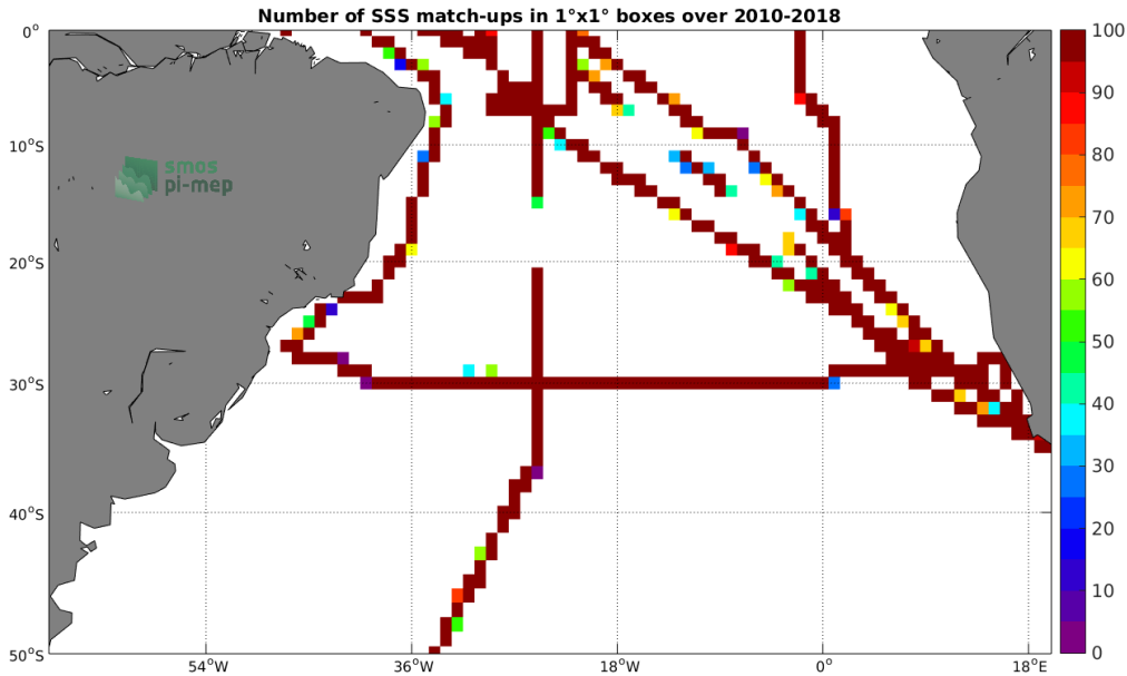
Figure 4: Number of SSS match-ups between TSG-SAMOS SSS and the SMOS-L3-CATDS-CPDC-V317-10DAYS-25KM SSS product for the South Atlantic Ocean Pi-MEP region over 1^\circ \times 1^\circ boxes and for the full satellite product period.
