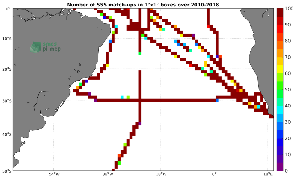
Figure 4: Number of SSS match-ups between TSG-SAMOS SSS and the SMOS-L3-CATDS-CPDC-V317-10DAYS-25KM SSS product for the South Atlantic Ocean Pi-MEP region over 1^{\circ} \times 1^{\circ} boxes and for the full satellite product period.
