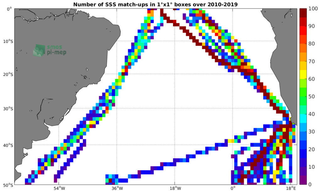
Figure 4: Number of SSS match-ups between TSG-POLARSTERN SSS and the SMOS L3 v317 - 10 Days - 25 km (CATDS-CPDC) SSS product for the South Atlantic Ocean Pi-MEP region over 1°x1° boxes and for the full satellite product period.
