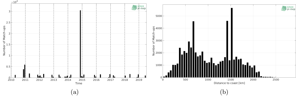
Figure 1: Number of match-ups between TSG-POLARSTERN and SMOS L3 v317 - 10 Days - 25 km (CATDS-CPDC) SSS as a function of time (a) and as function of the distance to coast (b) over the South Atlantic Ocean Pi-MEP region and for the full satellite product period.
