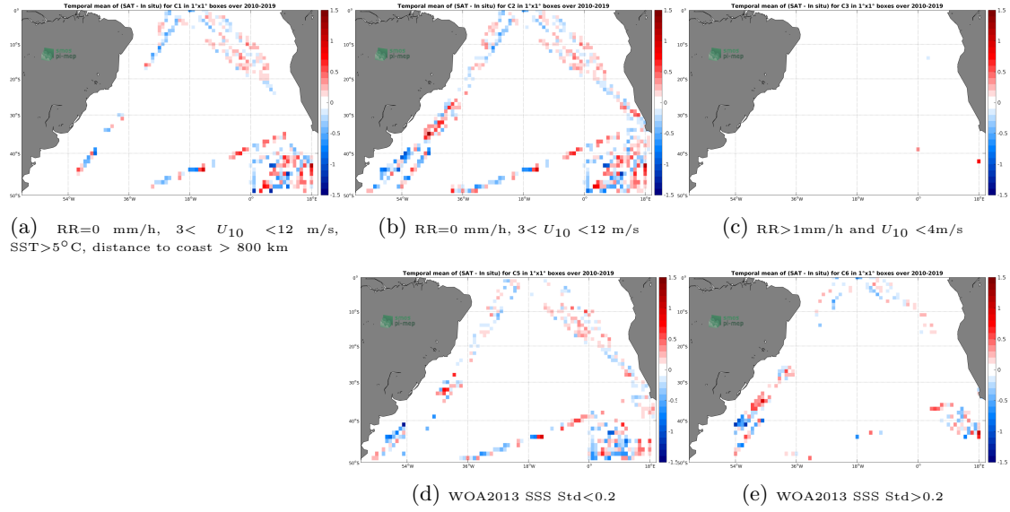
Figure 12: Temporal mean gridded over spatial boxes of size 1^\circ \times 1^\circ of \Delta SSS (SMOS L3 v317 - 10 Days - 25 km (CATDS-CPDC) - TSG-POLARSTERN) for 5 different subdatasets corresponding to: RR=0 mm/h, 3 < U_{10} < 12 m/s, SST > 5^\circ C , distance to coast > 800 km (a), RR=0 mm/h, 3 < U_{10} < 12 m/s (b), RR > 1 mm/h and U_{10} < 4 m/s (c), WOA2013 SSS Std < 0.2 (d), WOA2013 SSS Std > 0.2 (e).
