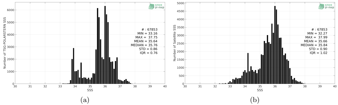
Figure 2: Histograms of SSS from TSG-POLARSTERN (a) and SMOS L3 v317 - 10 Days - 25 km (CATDS-CPDC) (b) considering all match-up pairs per bins of 0.1 over the South Atlantic Ocean Pi-MEP region and for the full satellite product period.
