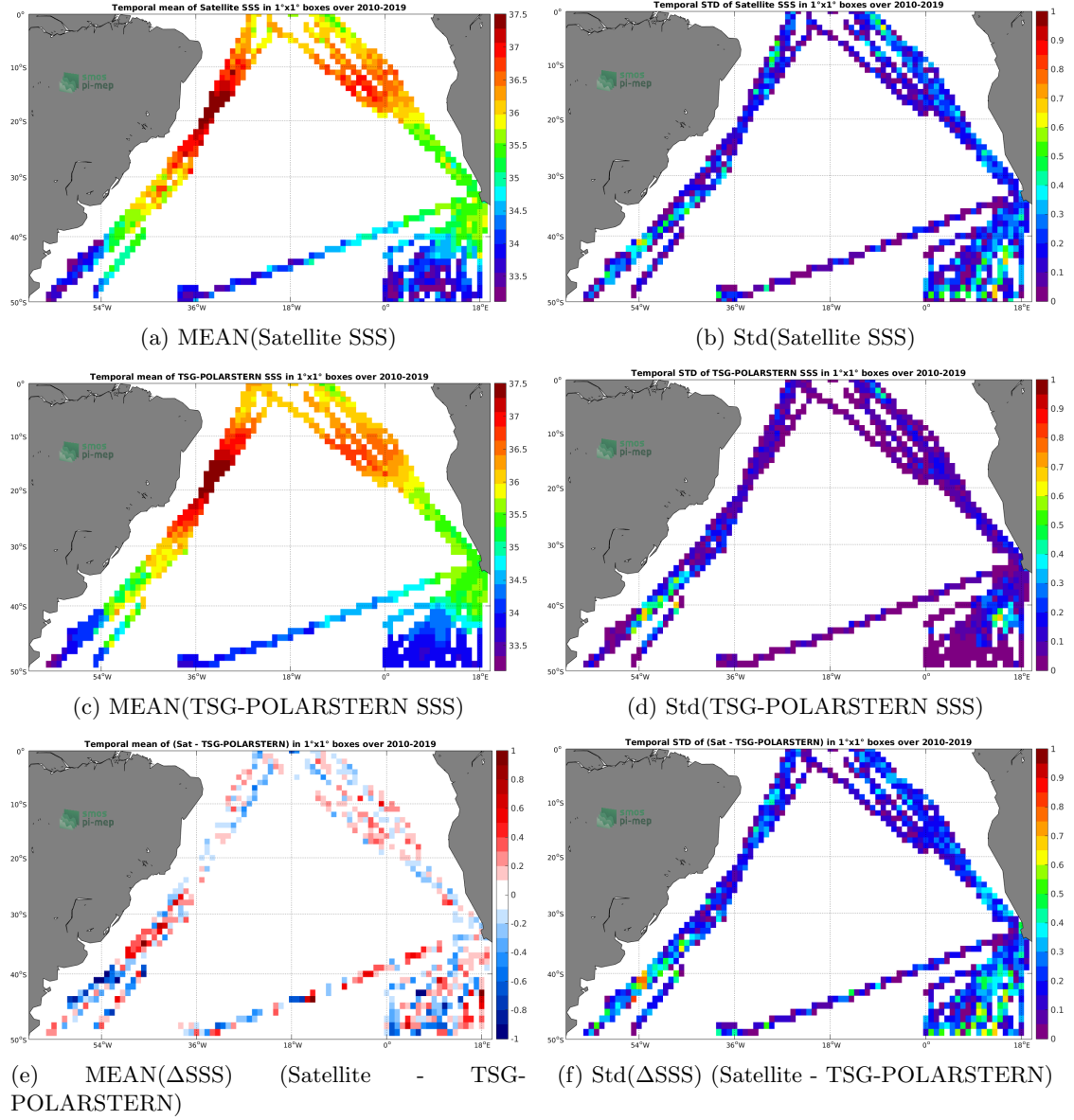
Figure 6: Temporal mean (left) and Std (right) of SSS from SMOS L3 v317 - 10 Days - 25 km (CATDS-CPDC) (top), TSG-POLARSTERN (middle), and of \Delta SSS (Satellite - TSG-POLARSTERN). Only match-up pairs are used to generate these maps.
