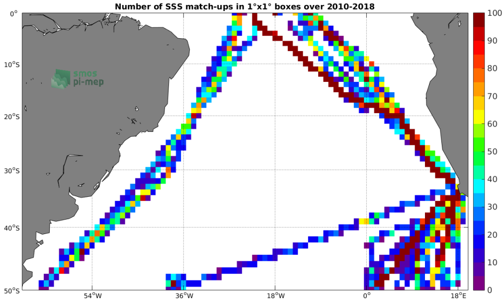
Figure 4: Number of SSS match-ups between TSG-POLARSTERN SSS and the SMOS-L3-CATDS-CPDC-V317-10DAYS-25KM SSS product for the South Atlantic Ocean Pi-MEP region over 1°x1° boxes and for the full satellite product period.
