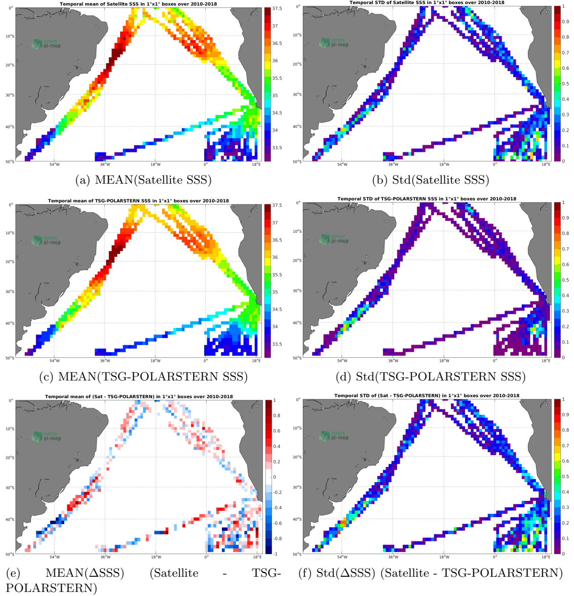
Figure 6: Temporal mean (left) and Std (right) of SSS from SMOS-L3-CATDS-CPDC-V317-10DAYS-25KM (top), TSG-POLARSTERN (middle), and of \Delta SSS (Satellite - TSG-POLARSTERN). Only match-up pairs are used to generate these maps.
