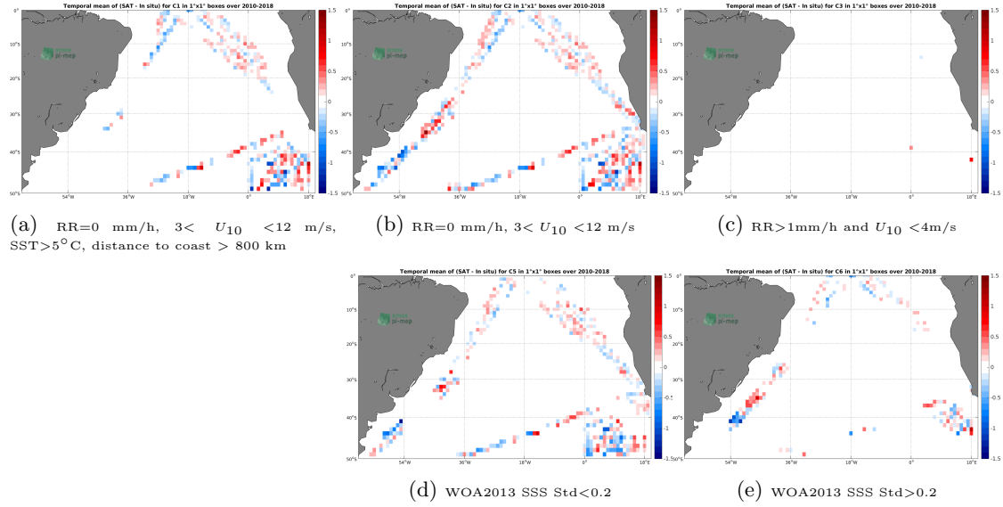
Figure 12: Temporal mean gridded over spatial boxes of size 1^\circ \times 1^\circ of \Delta SSS (SMOS-L3-CATDS-CPDC-V317-10DAYS-25KM - TSG-POLARSTERN) for 5 different subdatasets corresponding to: RR=0 mm/h, 3 < U_{10} < 12 m/s, SST > 5^\circ C , distance to coast > 800 km (a), RR=0 mm/h, 3 < U_{10} < 12 m/s (b), RR > 1 mm/h and U_{10} < 4 m/s (c), WOA2013 SSS Std < 0.2 (d), WOA2013 SSS Std > 0.2 (e).
