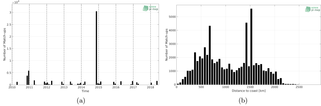
Figure 1: Number of match-ups between TSG-POLARSTERN and SMOS-L3-CATDS-CPDC-V317-10DAYS-25KM SSS as a function of time (a) and as function of the distance to coast (b) over the South Atlantic Ocean Pi-MEP region and for the full satellite product period.
