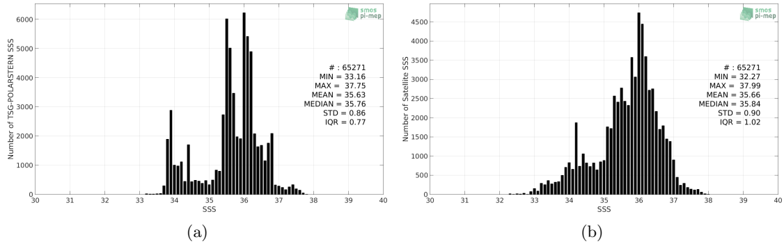
Figure 2: Histograms of SSS from TSG-POLARSTERN (a) and SMOS-L3-CATDS-CPDC-V317-10DAYS-25KM (b) considering all match-up pairs per bins of 0.1 over the South Atlantic Ocean Pi-MEP region and for the full satellite product period.
