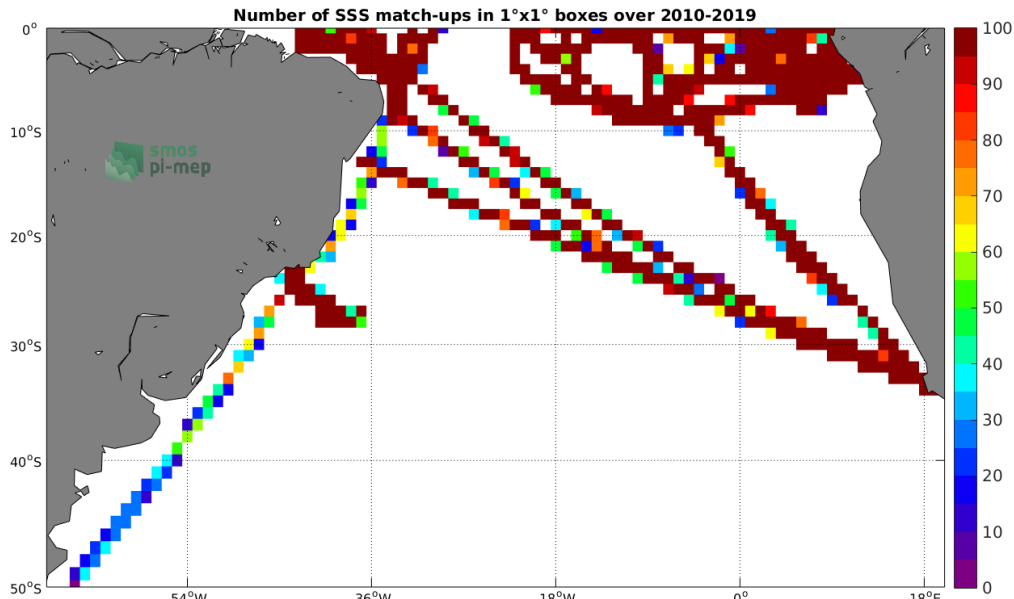
Figure 4: Number of SSS match-ups between TSG (GOSUD-Research-vessel) SSS and the SMOS SSS L3 v317 - 10 Days - 25 km (CATDS-CPDC) SSS product for the South Atlantic Ocean Pi-MEP region over 1^\circ \times 1^\circ boxes and for the full satellite product period.
