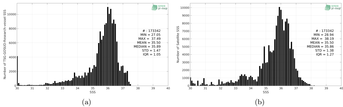
Figure 2: Histograms of SSS from TSG-GOSUD-Research-vessel (a) and SMOS-L3-CATDS-CPDC-V317-10DAYS-25KM (b) considering all match-up pairs per bins of 0.1 over the South Atlantic Ocean Pi-MEP region and for the full satellite product period.
