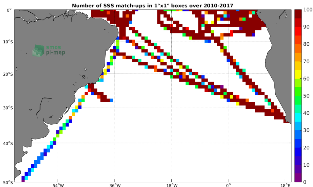
Figure 4: Number of SSS match-ups between TSG-GOSUD-Research-vessel SSS and the SMOS-L3-CATDS-CPDC-V317-10DAYS-25KM SSS product for the South Atlantic Ocean Pi-MEP region over 1°x1° boxes and for the full satellite product period.
