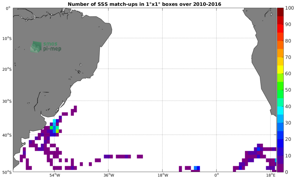
Figure 4: Number of SSS match-ups between Marine mammals SSS and the SMOS SSS L3 v317 - 10 Days - 25 km (CATDS-CPDC) SSS product for the South Atlantic Ocean Pi-MEP region over 1^\circ \times 1^\circ boxes and for the full satellite product period.
