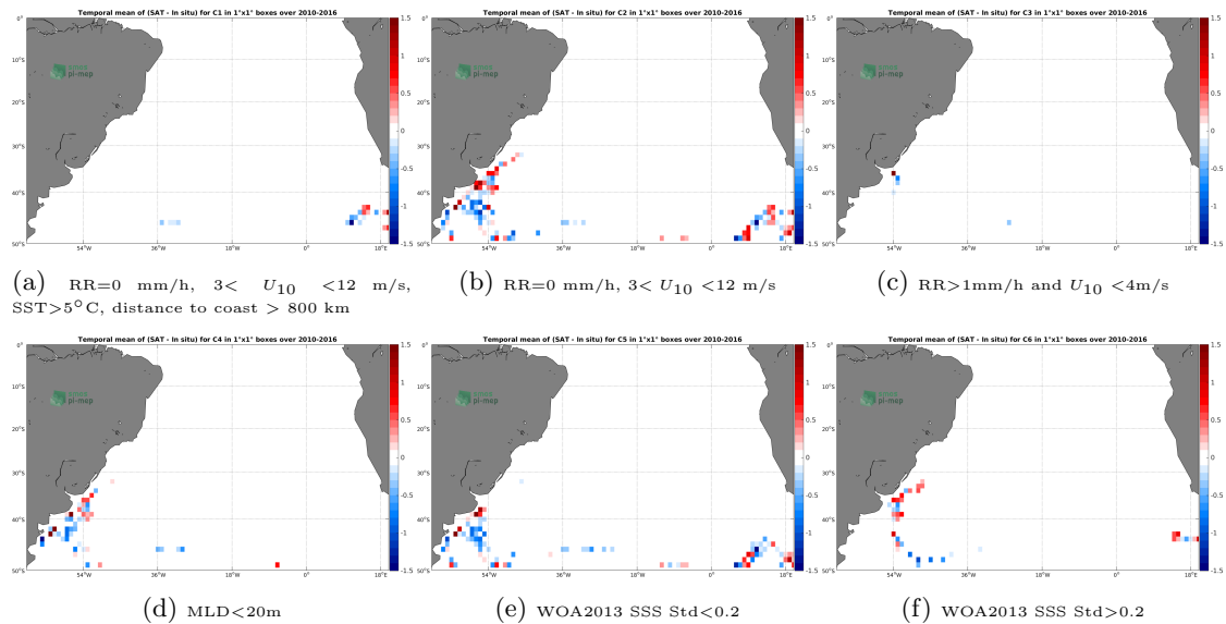
Figure 12: Temporal mean gridded over spatial boxes of size 1^\circ \times 1^\circ of \Delta SSS (SMOS SSS L3 v317 - 10 Days - 25 km (CATDS-CPDC) - Marine mammals) for 6 different subdatasets corresponding to:RR=0 mm/h, 3 < U_{10} < 12 m/s, SST >5^\circ C, distance to coast > 800 km (a), RR=0 mm/h, 3 < U_{10} < 12 m/s (b), RR >1 mm/h and U_{10} < 4 m/s (c),MLD <20 m (d),WOA2013 SSS Std <0.2 (e),WOA2013 SSS Std >0.2 (f).
