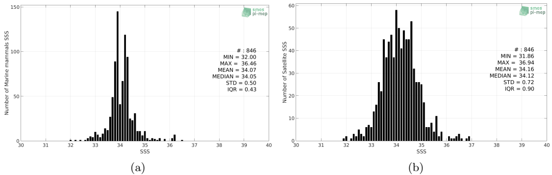
Figure 2: Histograms of SSS from Marine mammals (a) and SMOS SSS L3 v317 - 10 Days - 25 km (CATDS-CPDC) (b) considering all match-up pairs per bins of 0.1 over the South Atlantic Ocean Pi-MEP region and for the full satellite product period.
