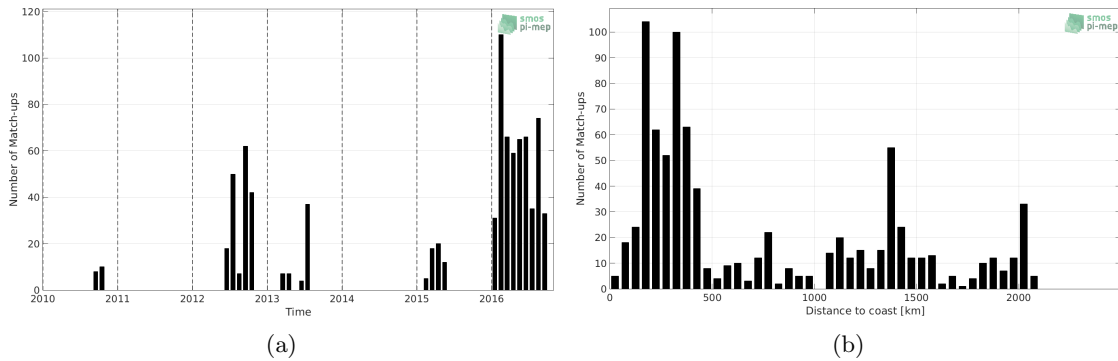
Figure 1: Number of match-ups between Marine mammals and SMOS SSS L3 v317 - 10 Days - 25 km (CATDS-CPDC) SSS as a function of time (a) and as function of the distance to coast (b) over the South Atlantic Ocean Pi-MEP region and for the full satellite product period.
