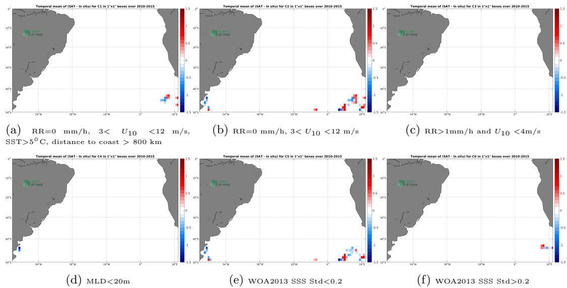
Figure 12: Temporal mean gridded over spatial boxes of size 1^\circ \times 1^\circ of \Delta SSS (SMOS-L3-CATDS-CPDC-V317-10DAYS-25KM - Sea mammals) for 6 different subdatasets corresponding to:RR=0 mm/h, 3 < U_{10} < 12 m/s, SST >5^\circ C, distance to coast > 800 km (a), RR=0 mm/h, 3 < U_{10} < 12 m/s (b), RR >1 mm/h and U_{10} < 4 m/s (c),MLD <20 m (d),WOA2013 SSS Std <0.2 (e),WOA2013 SSS Std >0.2 (f).
