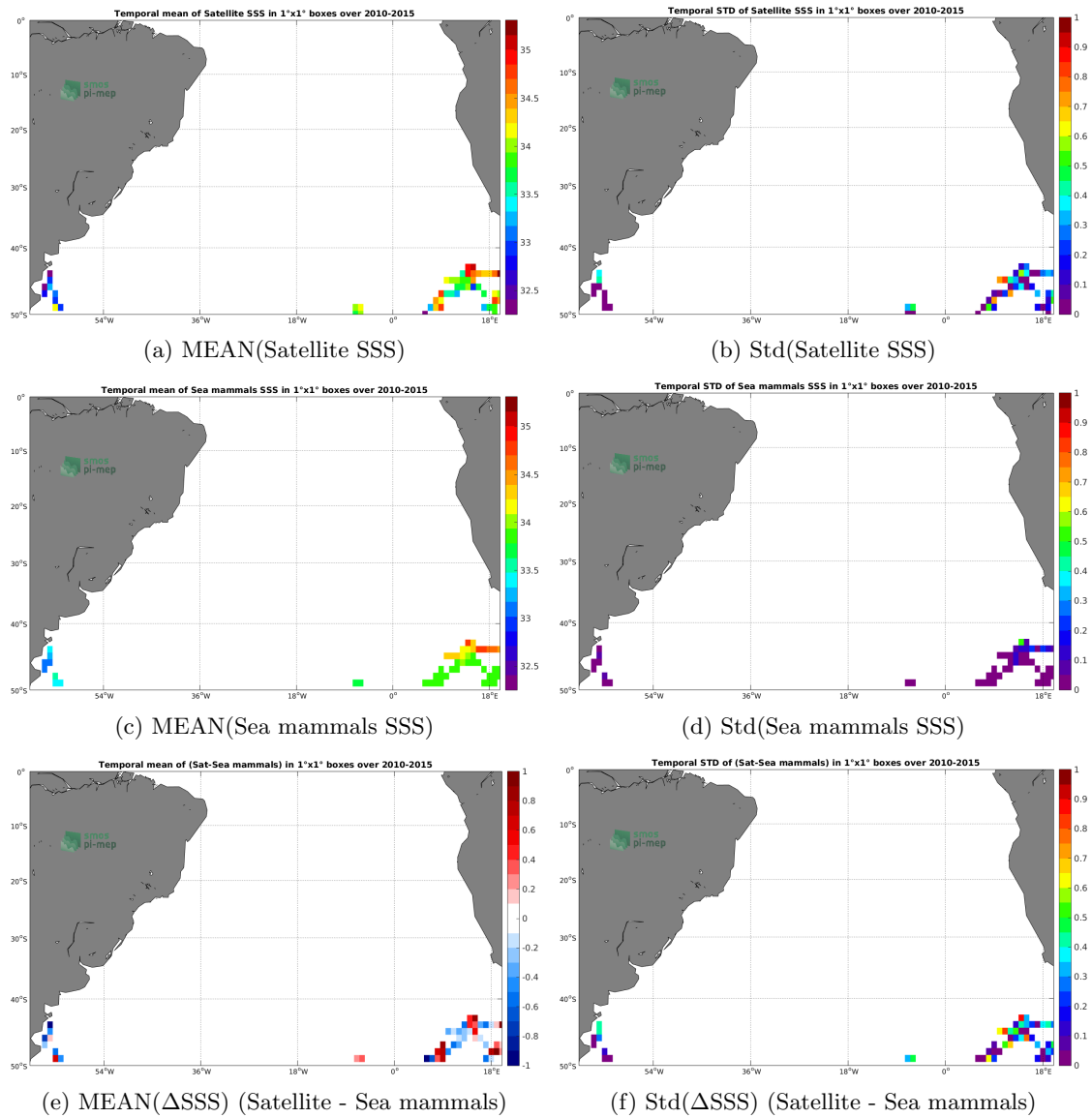
Figure 6: Temporal mean (left) and Std (right) of SSS from SMOS-L3-CATDS-CPDC-V317-10DAYS-25KM (top), Sea mammals (middle), and of \Delta SSS (Satellite - Sea mammals). Only match-up pairs are used to generate these maps.
