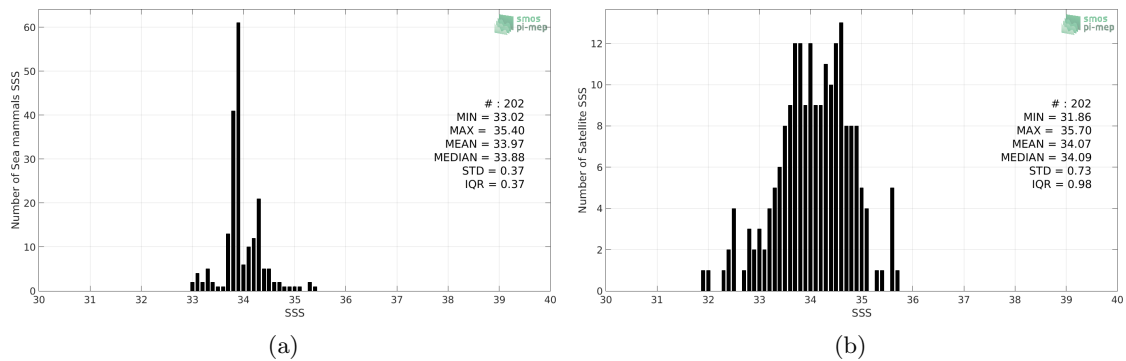
Figure 2: Histograms of SSS from Sea mammals (a) and SMOS-L3-CATDS-CPDC-V317-10DAYS-25KM (b) considering all match-up pairs per bins of 0.1 over the South Atlantic Ocean Pi-MEP region and for the full satellite product period.
