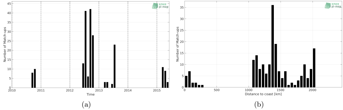
Figure 1: Number of match-ups between Sea mammals and SMOS-L3-CATDS-CPDC-V317-10DAYS-25KM SSS as a function of time (a) and as function of the distance to coast (b) over the South Atlantic Ocean Pi-MEP region and for the full satellite product period.
