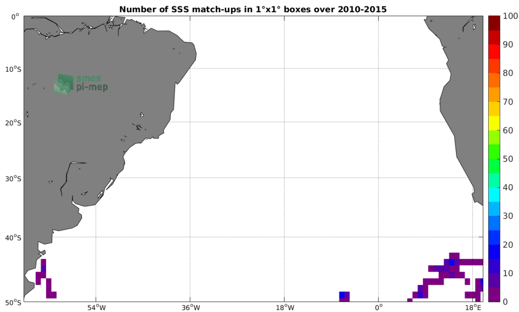
Figure 4: Number of SSS match-ups between Sea mammals SSS and the SMOS-L3-CATDS-CPDC-V317-10DAYS-25KM SSS product for the South Atlantic Ocean Pi-MEP region over 1^\circ \times 1^\circ boxes and for the full satellite product period.
