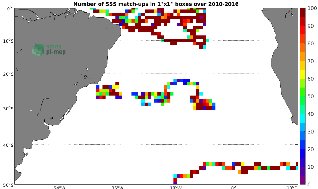
Figure 3: Number of SSS match-ups between Surface drifters SSS and the SMOS SSS L3 v317 - 10 Days - 25 km (CATDS-CPDC) SSS product for the South Atlantic Ocean Pi-MEP region over 1^\circ \times 1^\circ boxes and for the full satellite product period.
