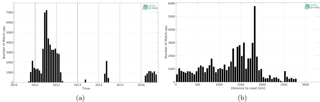
Figure 1: Number of match-ups between Surface drifters and SMOS SSS L3 v317 - 10 Days - 25 km (CATDS-CPDC) SSS as a function of time (a) and as function of the distance to coast (b) over the South Atlantic Ocean Pi-MEP region and for the full satellite product period.
