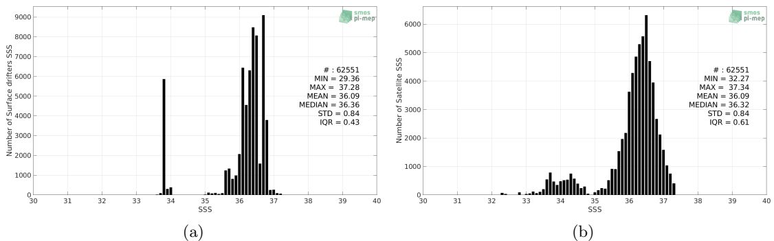
Figure 2: Histograms of SSS from Surface drifters (a) and SMOS SSS L3 v317 - 10 Days - 25 km (CATDS-CPDC) (b) considering all match-up pairs per bins of 0.1 over the South Atlantic Ocean Pi-MEP region and for the full satellite product period.
