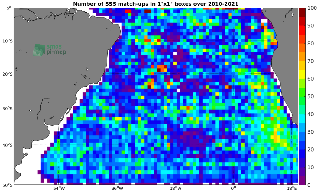
Figure 4: Number of SSS match-ups between Argo SSS and the SMOS SSS L3 v317 - 10 Days - 25 km (CATDS-CPDC) SSS product for the South Atlantic Ocean Pi-MEP region over 1^\circ \times 1^\circ boxes and for the full satellite product period.
