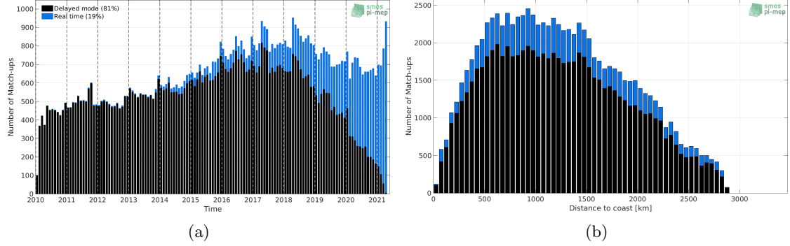
Figure 1: Number of match-ups between Argo and SMOS SSS L3 v317 - 10 Days - 25 km (CATDS-CPDC) SSS as a function of time (a) and as function of the distance to coast (b) over the South Atlantic Ocean Pi-MEP region and for the full satellite product period.
