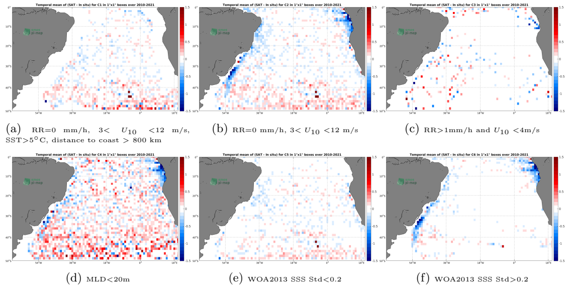
Figure 12: Temporal mean gridded over spatial boxes of size 1^\circ \times 1^\circ of \Delta SSS (SMOS SSS L3 v317 - 10 Days - 25 km (CATDS-CPDC) - Argo) for 6 different subdatasets corresponding to: RR=0 mm/h, 3 < U_{10} < 12 m/s, SST > 5^\circ C , distance to coast > 800 km (a), RR=0 mm/h, 3 < U_{10} < 12 m/s (b), RR > 1 mm/h and U_{10} < 4 m/s (c), MLD < 20 m (d), WOA2013 SSS Std < 0.2 (e), WOA2013 SSS Std > 0.2 (f).
