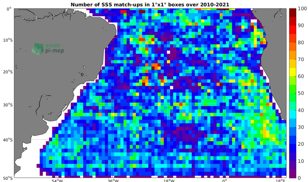
Figure 4: Number of SSS match-ups between Argo SSS and the SMOS SSS L3 v317 - 10 Days - 25 km (CATDS-CPDC) SSS product for the South Atlantic Ocean Pi-MEP region over 1^\circ \times 1^\circ boxes and for the full satellite product period.
