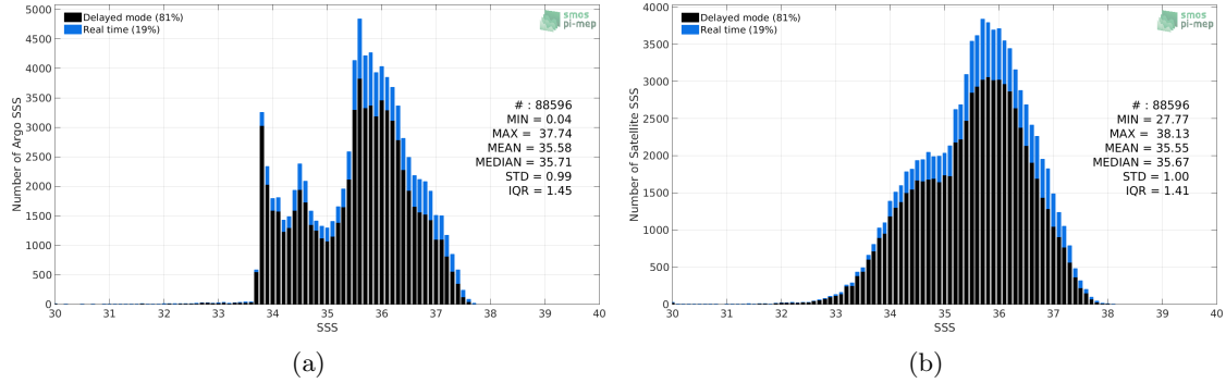
Figure 2: Histograms of SSS from Argo (a) and SMOS SSS L3 v317 - 10 Days - 25 km (CATDS-CPDC) (b) considering all match-up pairs per bins of 0.1 over the South Atlantic Ocean Pi-MEP region and for the full satellite product period.
