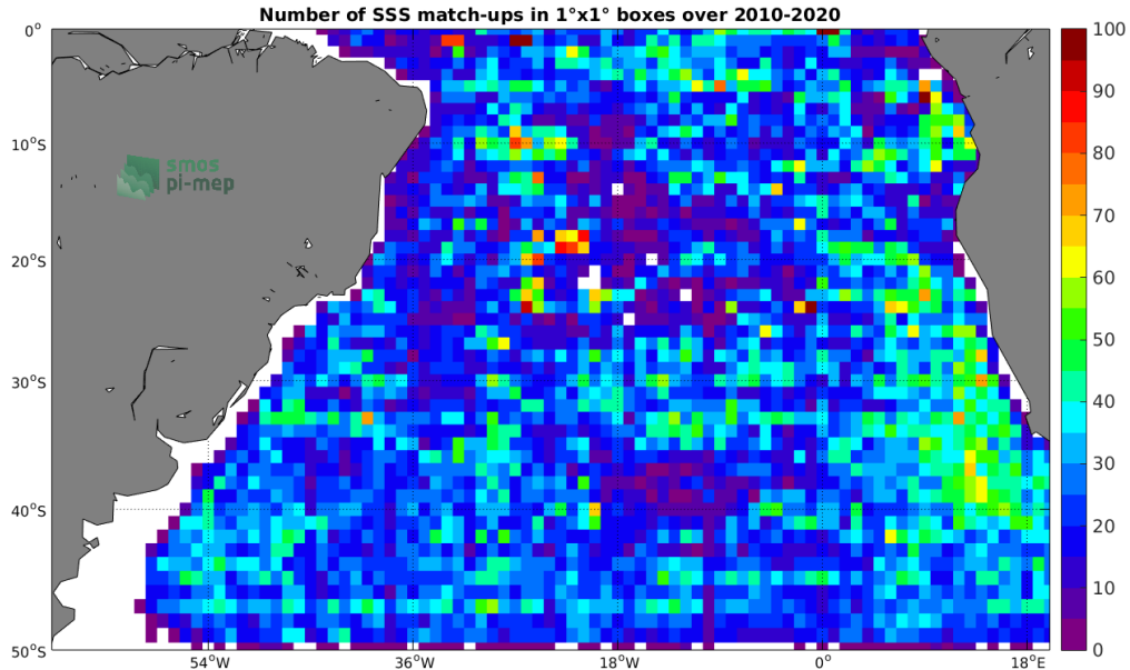
Figure 4: Number of SSS match-ups between Argo SSS and the SMOS L3 v317 - 10 Days - 25 km (CATDS-CPDC) SSS product for the South Atlantic Ocean Pi-MEP region over 1°x1° boxes and for the full satellite product period.
