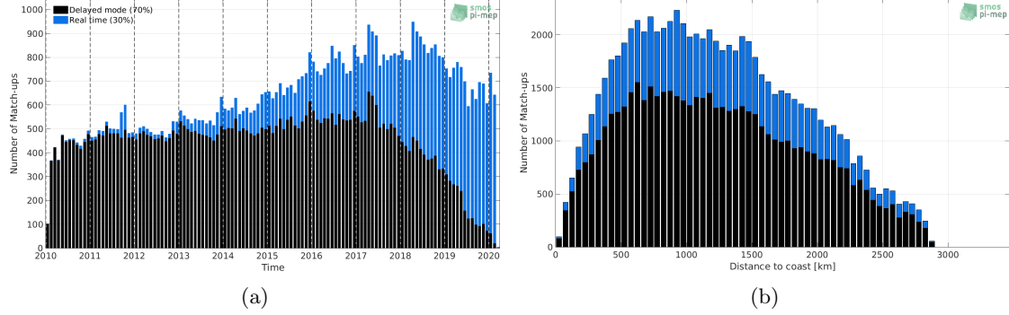
Figure 1: Number of match-ups between Argo and SMOS L3 v317 - 10 Days - 25 km (CATDS-CPDC) SSS as a function of time (a) and as function of the distance to coast (b) over the South Atlantic Ocean Pi-MEP region and for the full satellite product period.
