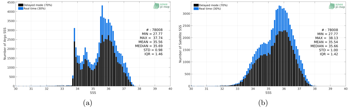
Figure 2: Histograms of SSS from Argo (a) and SMOS L3 v317 - 10 Days - 25 km (CATDS-CPDC) (b) considering all match-up pairs per bins of 0.1 over the South Atlantic Ocean Pi-MEP region and for the full satellite product period.
