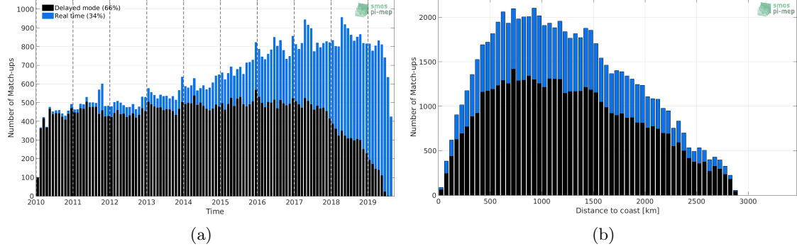
Figure 1: Number of match-ups between Argo and SMOS-L3-CATDS-CPDC-V317-10DAYS-25KM SSS as a function of time (a) and as function of the distance to coast (b) over the South Atlantic Ocean Pi-MEP region and for the full satellite product period.
