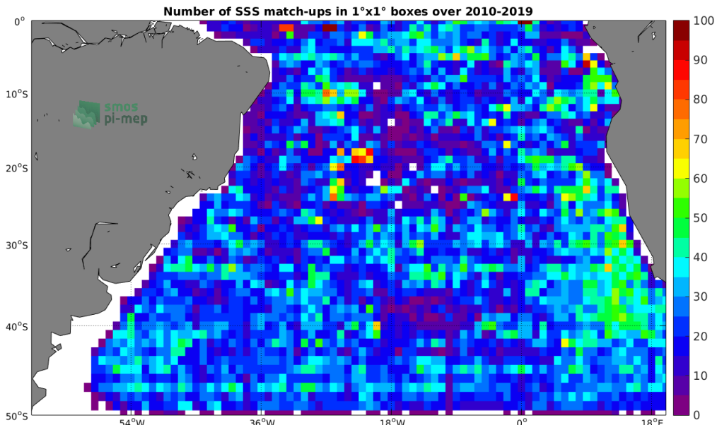
Figure 4: Number of SSS match-ups between Argo SSS and the SMOS-L3-CATDS-CPDC-V317-10DAYS-25KM SSS product for the South Atlantic Ocean Pi-MEP region over 1°x1° boxes and for the full satellite product period.
