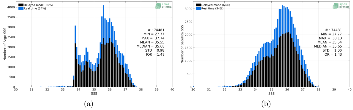
Figure 2: Histograms of SSS from Argo (a) and SMOS-L3-CATDS-CPDC-V317-10DAYS-25KM (b) considering all match-up pairs per bins of 0.1 over the South Atlantic Ocean Pi-MEP region and for the full satellite product period.
