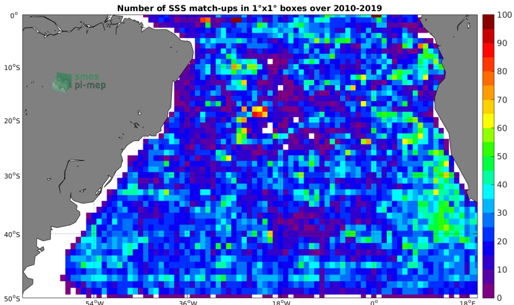
Figure 4: Number of SSS match-ups between Argo SSS and the SMOS-L3-CATDS-CPDC-V317-10DAYS-25KM SSS product for the South Atlantic Ocean Pi-MEP region over 1^\circ \times 1^\circ boxes and for the full satellite product period.
