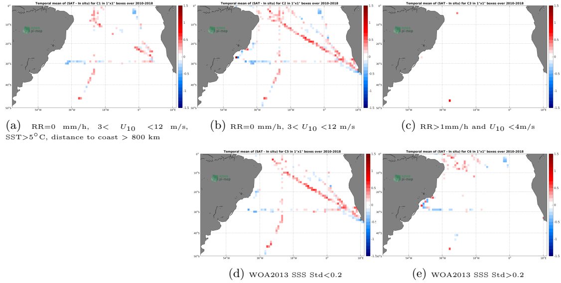
Figure 12: Temporal mean gridded over spatial boxes of size 1^\circ \times 1^\circ of \Delta SSS (SMOS-L3-CATDS-CPDC-V3-MONTHLY-25KM - TSG-SAMOS) for 5 different subdatasets corresponding to: RR=0 mm/h, 3 < U_{10} < 12 m/s, SST > 5^\circ\text{C} , distance to coast > 800 km (a), RR=0 mm/h, 3 < U_{10} < 12 m/s (b), RR > 1 mm/h and U_{10} < 4 m/s (c), WOA2013 SSS Std < 0.2 (d), WOA2013 SSS Std > 0.2 (e).
