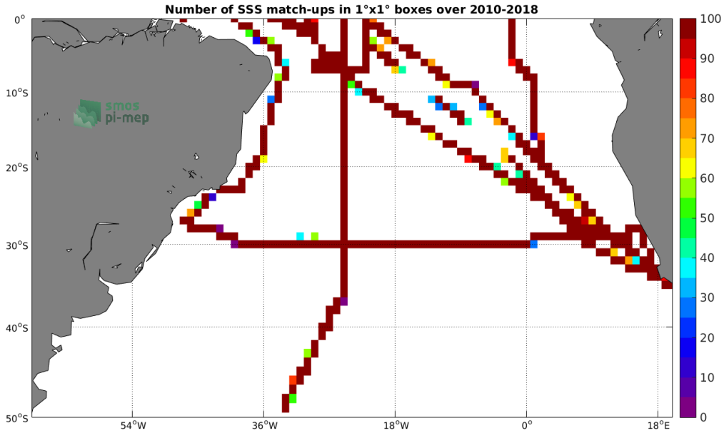
Figure 4: Number of SSS match-ups between TSG-SAMOS SSS and the SMOS-L3-CATDS-CPDC-V3-MONTHLY-25KM SSS product for the South Atlantic Ocean Pi-MEP region over 1^\circ \times 1^\circ boxes and for the full satellite product period.
