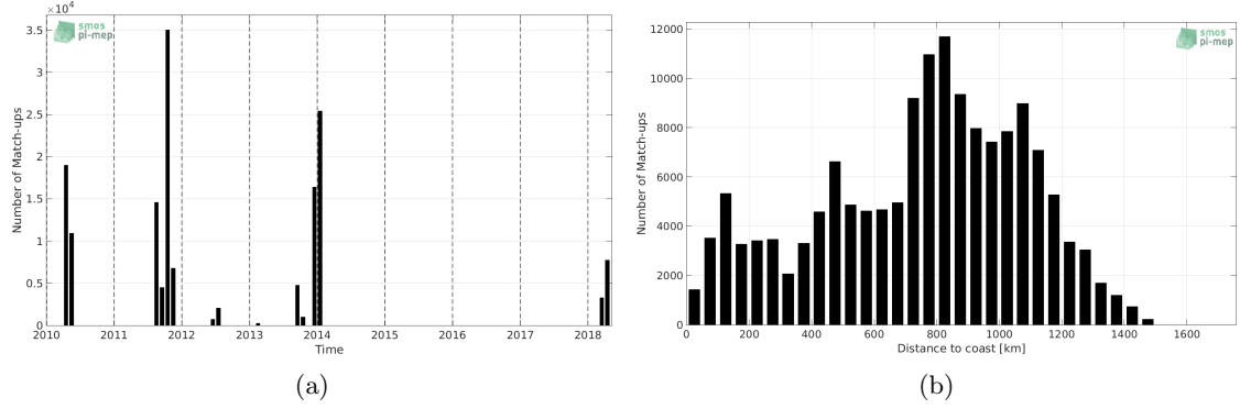
Figure 1: Number of match-ups between TSG-SAMOS and SMOS-L3-CATDS-CPDC-V3-MONTHLY-25KM SSS as a function of time (a) and as function of the distance to coast (b) over the South Atlantic Ocean Pi-MEP region and for the full satellite product period.
