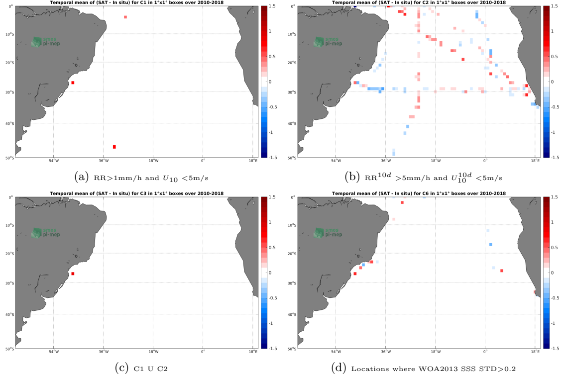
Figure 12: Temporal mean gridded over spatial boxes of size 1^\circ \times 1^\circ of \Delta SSS (SMOS-L3-CATDS-CPDC-V3-MONTHLY-25KM - TSG-SAMOS) for 4 different subdatasets corresponding to: RR > 1mm/h and U_{10} < 5\text{m/s} (a), RR^{10d} > 5\text{mm/h} and U_{10}^{10d} < 5\text{m/s} (b), C1 U C2 (c), Locations where WOA2013 SSS STD > 0.2 (d).
