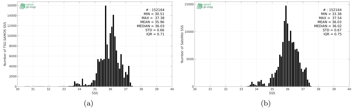
Figure 2: Histograms of SSS from TSG-SAMOS (a) and SMOS-L3-CATDS-CPDC-V3-MONTHLY-25KM (b) considering all match-up pairs per bins of 0.1 over the South Atlantic Ocean Pi-MEP region and for the full satellite product period.
