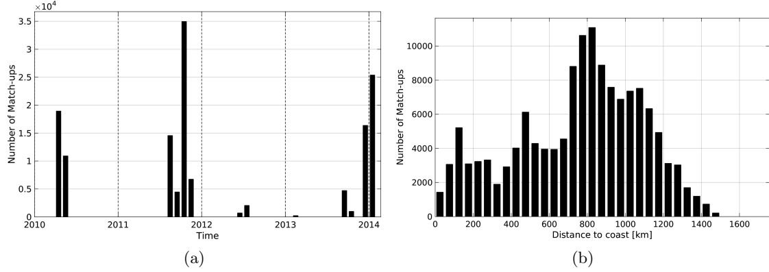
Figure 1: Number of match-ups between TSG-SAMOS and SMOS-L3-CATDS-CPDC-V3-MONTHLY-25KM SSS as a function of time (a) and as function of the distance to coast (b) over the South Atlantic Ocean Pi-MEP region and for the full satellite product period.
