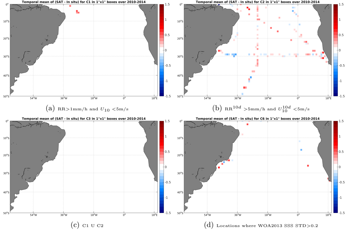
Figure 12: Temporal mean gridded over spatial boxes of size 1^\circ \times 1^\circ of \Delta SSS (SMOS-L3-CATDS-CPDC-V3-MONTHLY-25KM - TSG-SAMOS) for 4 different subdatasets corresponding to: RR > 1\text{mm/h} and U_{10} < 5\text{m/s} (a), RR^{10d} > 5\text{mm/h} and U_{10}^{10d} < 5\text{m/s} (b), C1 U C2 (c), Locations where WOA2013 SSS STD > 0.2 (d).
