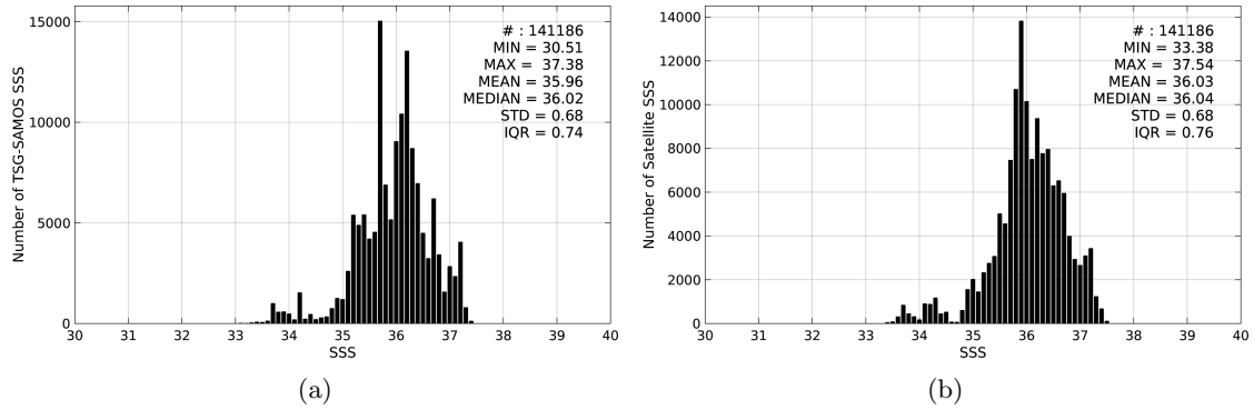
Figure 2: Histograms of SSS from TSG-SAMOS (a) and SMOS-L3-CATDS-CPDC-V3-MONTHLY-25KM (b) considering all match-up pairs per bins of 0.1 over the South Atlantic Ocean Pi-MEP region and for the full satellite product period.
