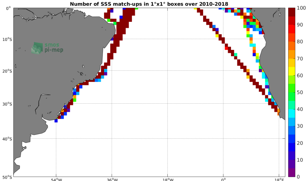
Figure 4: Number of SSS match-ups between TSG-LEGOS-DM SSS and the SMOS-L3-CATDS-CPDC-V3-MONTHLY-25KM SSS product for the South Atlantic Ocean Pi-MEP region over 1^\circ \times 1^\circ boxes and for the full satellite product period.
