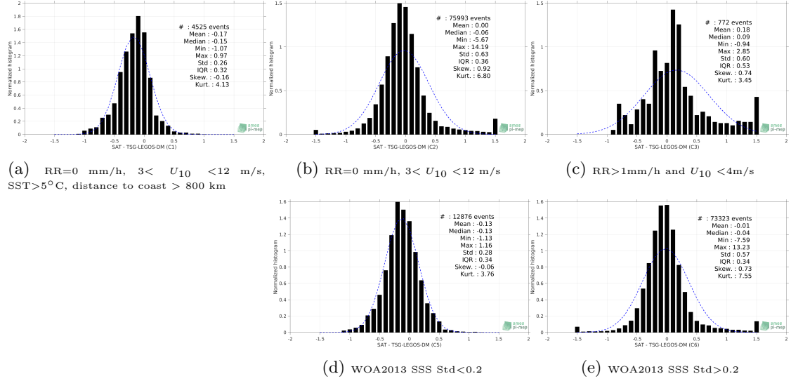
Figure 13: Normalized histogram of \Delta\text{SSS} (SMOS-L3-CATDS-CPDC-V3-MONTHLY-25KM - TSG-LEGOS-DM) for 5 different subdatasets corresponding to: RR=0 mm/h, 3 < U_{10} < 12 m/s, SST > 5^{\circ}\text{C} , distance to coast > 800 km (a), RR=0 mm/h, 3 < U_{10} < 12 m/s (b), RR > 1\text{mm/h} and U_{10} < 4\text{m/s} (c), WOA2013 SSS Std < 0.2 (d), WOA2013 SSS Std > 0.2 (e).
