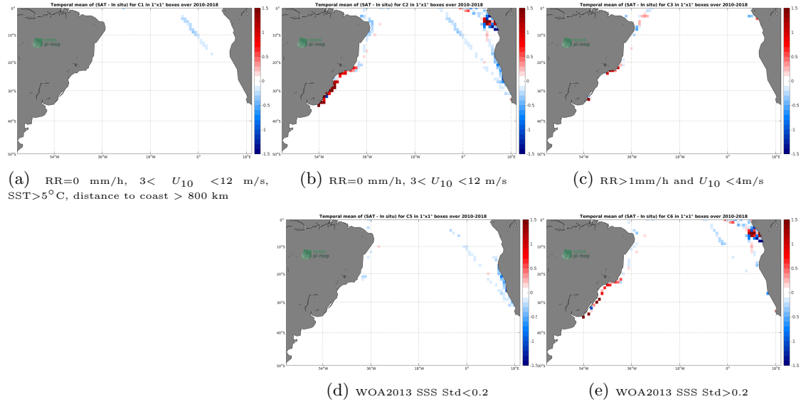
Figure 12: Temporal mean gridded over spatial boxes of size 1^\circ \times 1^\circ of \Delta SSS (SMOS-L3-CATDS-CPDC-V3-MONTHLY-25KM - TSG-LEGOS-DM) for 5 different subdatasets corresponding to: RR=0 mm/h, 3 < U_{10} < 12 m/s, SST > 5^\circ\text{C} , distance to coast > 800 km (a), RR=0 mm/h, 3 < U_{10} < 12 m/s (b), RR > 1 mm/h and U_{10} < 4 m/s (c), WOA2013 SSS Std < 0.2 (d), WOA2013 SSS Std > 0.2 (e).
