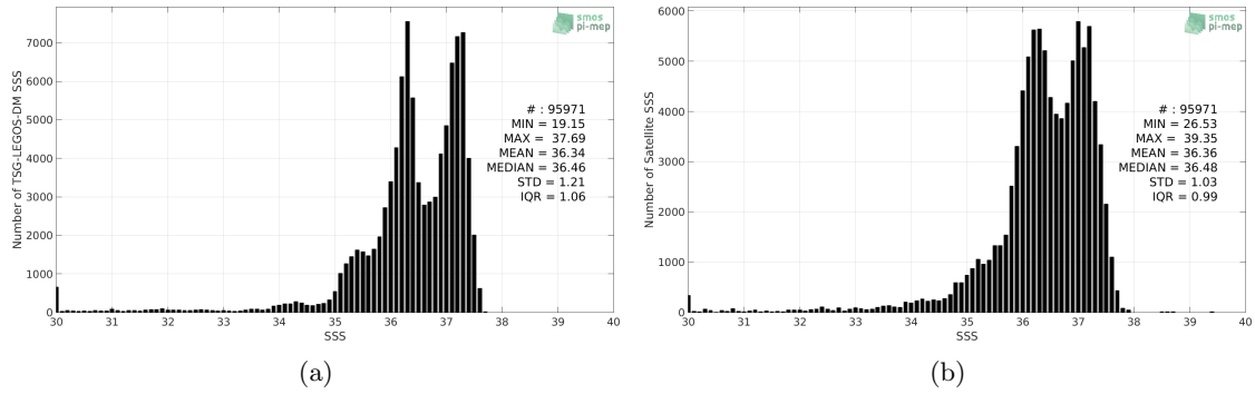
Figure 2: Histograms of SSS from TSG-LEGOS-DM (a) and SMOS-L3-CATDS-CPDC-V3-MONTHLY-25KM (b) considering all match-up pairs per bins of 0.1 over the South Atlantic Ocean Pi-MEP region and for the full satellite product period.
