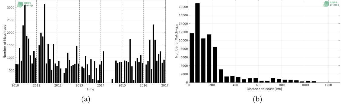
Figure 1: Number of match-ups between TSG-LEGOS-DM and SMOS-L3-CATDS-CPDC-V3-MONTHLY-25KM SSS as a function of time (a) and as function of the distance to coast (b) over the South Atlantic Ocean Pi-MEP region and for the full satellite product period.
