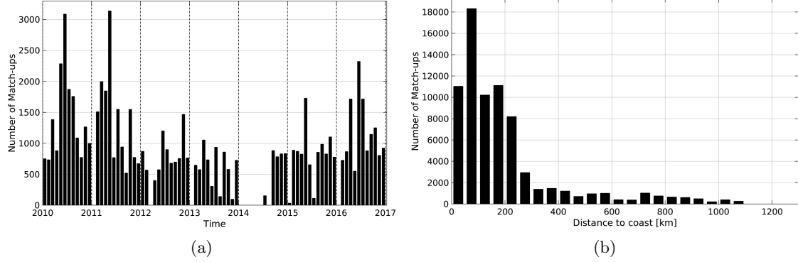
Figure 1: Number of match-ups between TSG-LEGOS-DM and SMOS-L3-CATDS-CPDC-V3-MONTHLY-25KM SSS as a function of time (a) and as function of the distance to coast (b) over the South Atlantic Ocean Pi-MEP region and for the full satellite product period.
