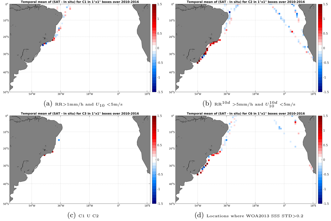
Figure 12: Temporal mean gridded over spatial boxes of size 1^\circ \times 1^\circ of \Delta SSS (SMOS-L3-CATDS-CPDC-V3-MONTHLY-25KM - TSG-LEGOS-DM) for 4 different subdatasets corresponding to: RR > 1\text{mm/h} and U_{10} < 5\text{m/s} (a), RR^{10d} > 5\text{mm/h} and U_{10}^{10d} < 5\text{m/s} (b), C1 U C2 (c), Locations where WOA2013 SSS STD > 0.2 (d).
