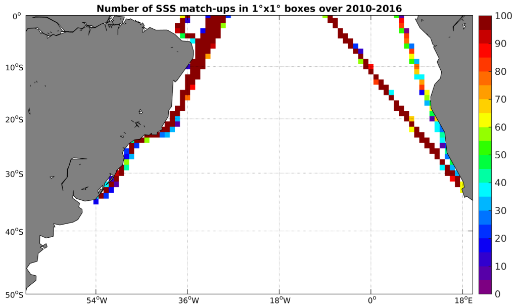
Figure 4: Number of SSS match-ups between TSG-LEGOS-DM SSS and the SMOS-L3-CATDS-CPDC-V3-MONTHLY-25KM SSS product for the South Atlantic Ocean Pi-MEP region over 1^\circ \times 1^\circ boxes and for the full satellite product period.
