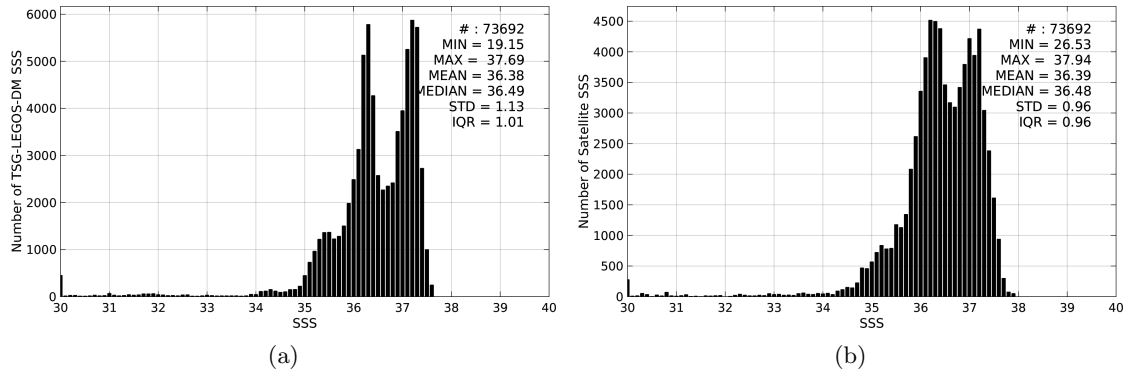
Figure 2: Histograms of SSS from TSG-LEGOS-DM (a) and SMOS-L3-CATDS-CPDC-V3-MONTHLY-25KM (b) considering all match-up pairs per bins of 0.1 over the South Atlantic Ocean Pi-MEP region and for the full satellite product period.
