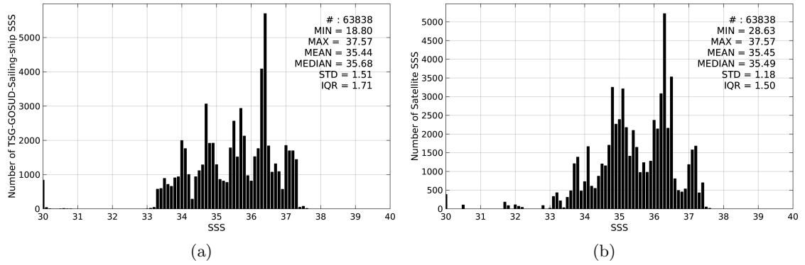
Figure 2: Histograms of SSS from TSG-GOSUD-Sailing-ship (a) and SMOS-L3-CATDS-CPDC-V3-MONTHLY-25KM (b) considering all match-up pairs per bins of 0.1 over the South Atlantic Ocean Pi-MEP region and for the full satellite product period.
