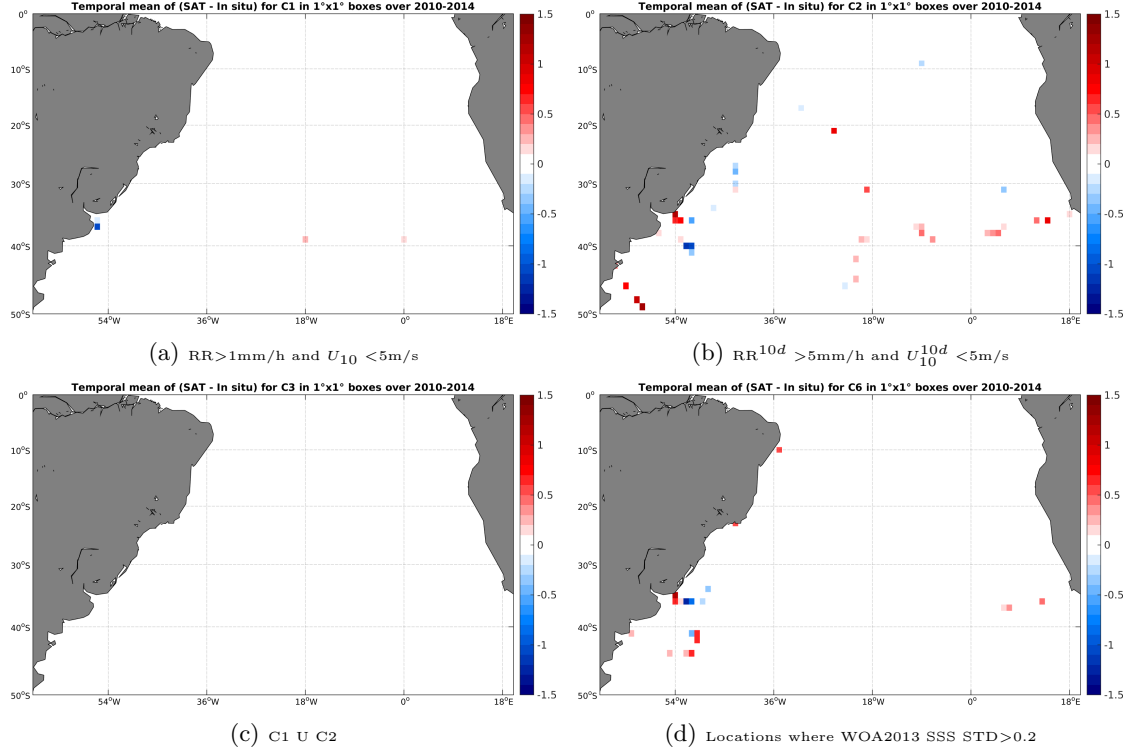
Figure 12: Temporal mean gridded over spatial boxes of size 1^\circ \times 1^\circ of \Delta SSS (SMOS-L3-CATDS-CPDC-V3-MONTHLY-25KM - TSG-GOSUD-Sailing-ship) for 4 different subdatasets corresponding to: RR > 1\text{mm/h} and U_{10} < 5\text{m/s} (a), RR^{10d} > 5\text{mm/h} and U_{10}^{10d} < 5\text{m/s} (b), C1 U C2 (c), Locations where WOA2013 SSS STD > 0.2 (d).
