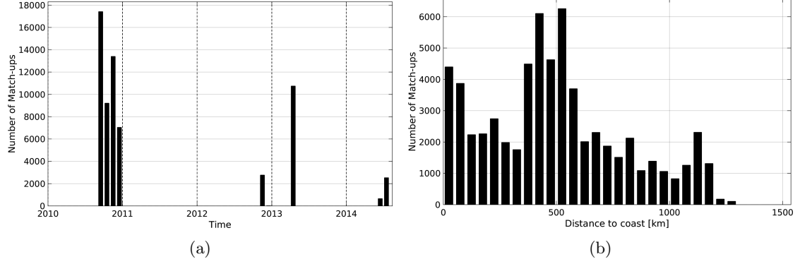
Figure 1: Number of match-ups between TSG-GOSUD-Sailing-ship and SMOS-L3-CATDS-CPDC-V3-MONTHLY-25KM SSS as a function of time (a) and as function of the distance to coast (b) over the South Atlantic Ocean Pi-MEP region and for the full satellite product period.
