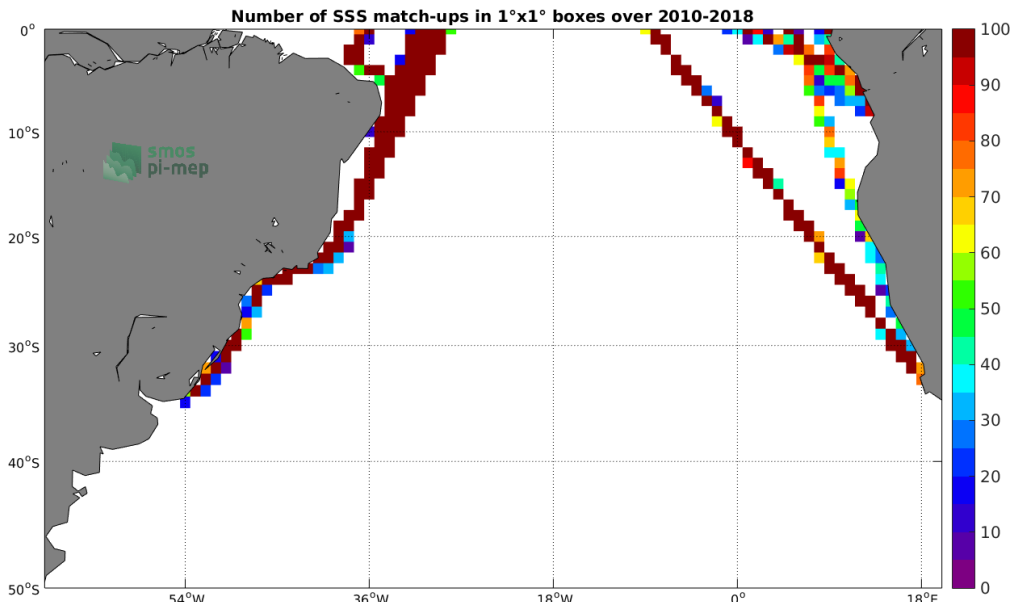
Figure 4: Number of SSS match-ups between TSG-LEGOS-DM SSS and the SMOS-L3-CATDS-CPDC-V3-10DAYS-25KM SSS product for the South Atlantic Ocean Pi-MEP region over 1^\circ \times 1^\circ boxes and for the full satellite product period.
