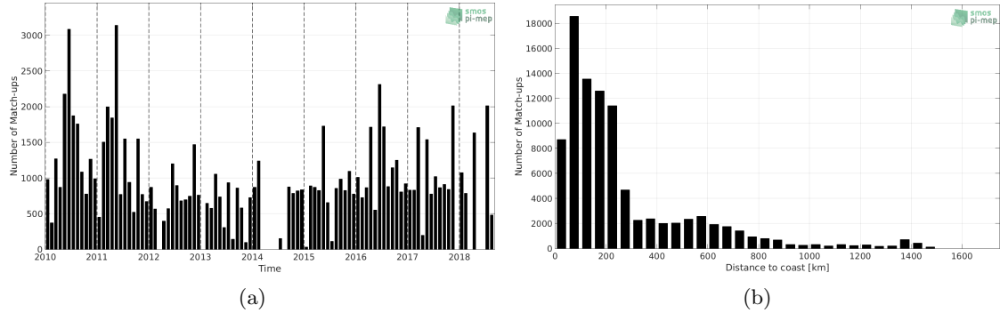
Figure 1: Number of match-ups between TSG-LEGOS-DM and SMOS-L3-CATDS-CPDC-V3-10DAYS-25KM SSS as a function of time (a) and as function of the distance to coast (b) over the South Atlantic Ocean Pi-MEP region and for the full satellite product period.
