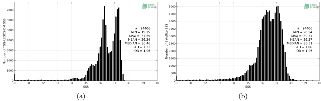
Figure 2: Histograms of SSS from TSG-LEGOS-DM (a) and SMOS-L3-CATDS-CPDC-V3-10DAYS-25KM (b) considering all match-up pairs per bins of 0.1 over the South Atlantic Ocean Pi-MEP region and for the full satellite product period.
