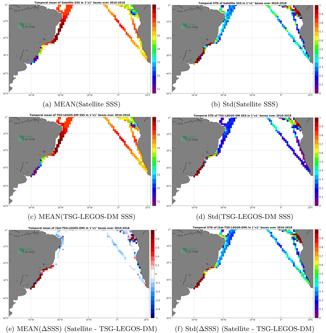
Figure 6: Temporal mean (left) and Std (right) of SSS from SMOS-L3-CATDS-CPDC-V3-10DAYS-25KM (top), TSG-LEGOS-DM (middle), and of \Delta SSS (Satellite - TSG-LEGOS-DM). Only match-up pairs are used to generate these maps.
