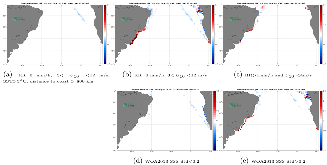
Figure 12: Temporal mean gridded over spatial boxes of size 1^\circ \times 1^\circ of \Delta SSS (SMOS-L3-CATDS-CPDC-V3-10DAYS-25KM - TSG-LEGOS-DM) for 5 different subdatasets corresponding to:RR=0 mm/h, 3 < U_{10} < 12 m/s, SST >5^\circ\text{C} , distance to coast > 800 km (a), RR=0 mm/h, 3 < U_{10} < 12 m/s (b), RR >1 mm/h and U_{10} < 4 m/s (c), WOA2013 SSS Std <0.2 (d), WOA2013 SSS Std >0.2 (e).
