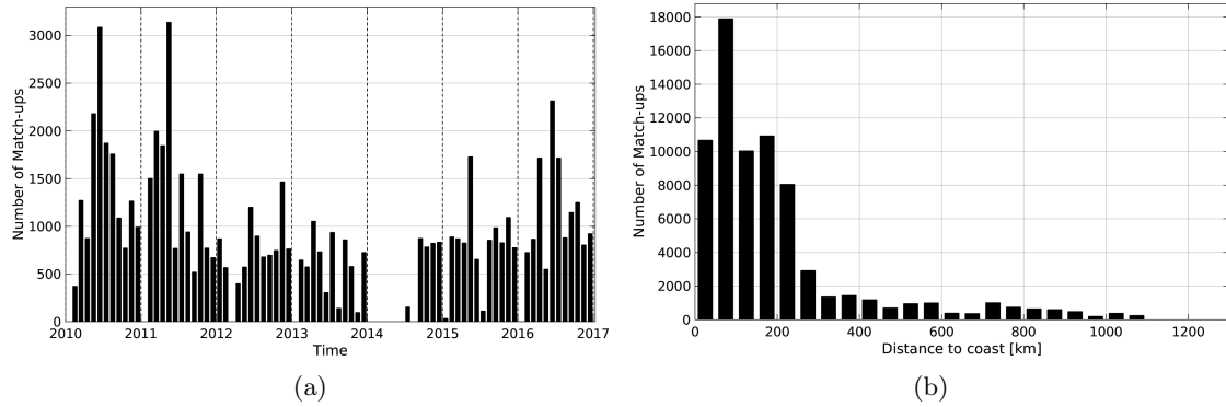
Figure 1: Number of match-ups between TSG-LEGOS-DM and SMOS-L3-CATDS-CPDC-V3-10DAYS-25KM SSS as a function of time (a) and as function of the distance to coast (b) over the South Atlantic Ocean Pi-MEP region and for the full satellite product period.
