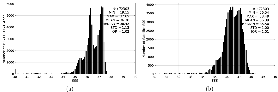
Figure 2: Histograms of SSS from TSG-LEGOS-DM (a) and SMOS-L3-CATDS-CPDC-V3-10DAYS-25KM (b) considering all match-up pairs per bins of 0.1 over the South Atlantic Ocean Pi-MEP region and for the full satellite product period.
