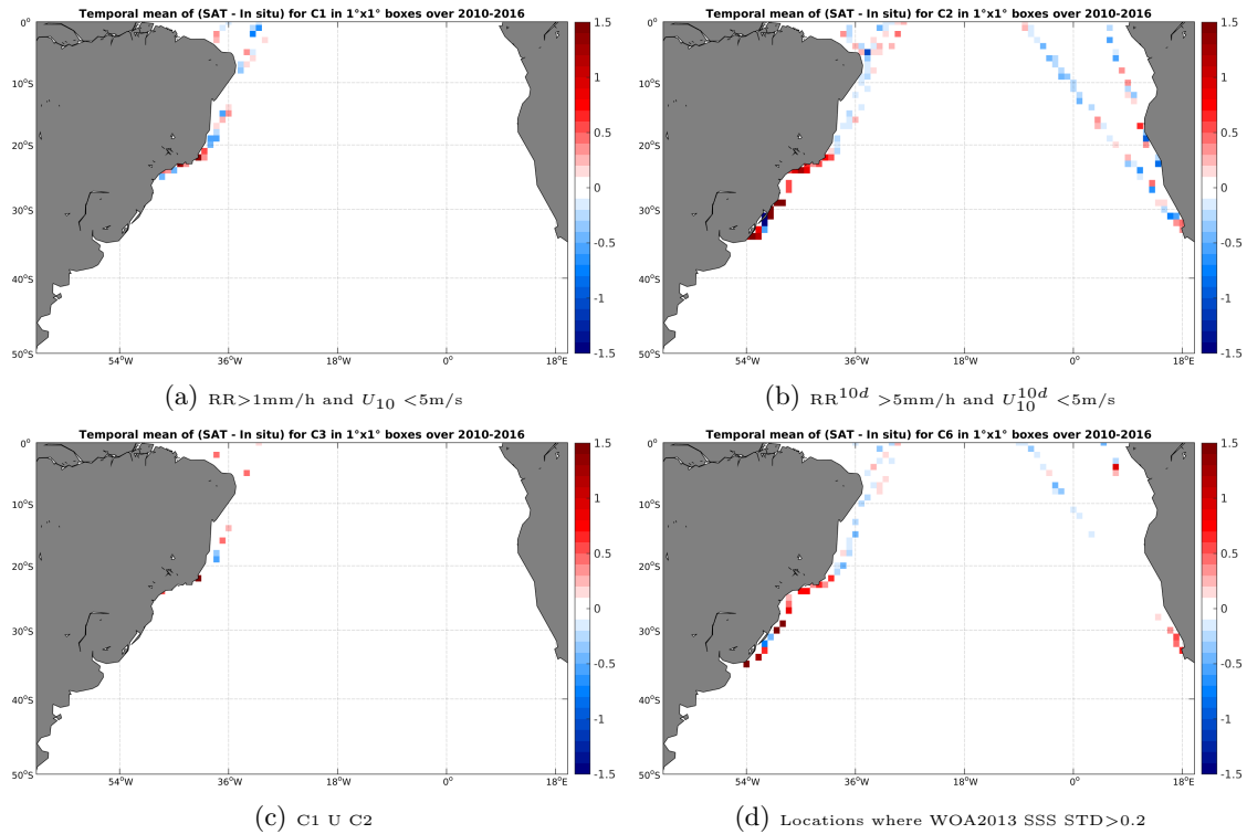
Figure 12: Temporal mean gridded over spatial boxes of size 1^\circ \times 1^\circ of \Delta SSS (SMOS-L3-CATDS-CPDC-V3-10DAYS-25KM - TSG-LEGOS-DM) for 4 different subdatasets corresponding to: RR > 1 mm/h and U_{10} < 5 m/s (a), RR 10d > 5 mm/h and U_{10}^{10d} < 5 m/s (b), C1 U C2 (c), Locations where WOA2013 SSS STD > 0.2 (d).
