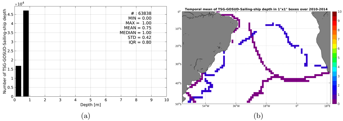
Figure 3: Histograms of the depth of the upper level SSS measurements from TSG-GOSUD-Sailing-ship in the Match-up DataBase for the South Atlantic Ocean Pi-MEP region (a) and temporal mean spatial distribution of pressure of the in situ SSS data over 1^\circ \times 1^\circ boxes and for the full satellite product period (b).
