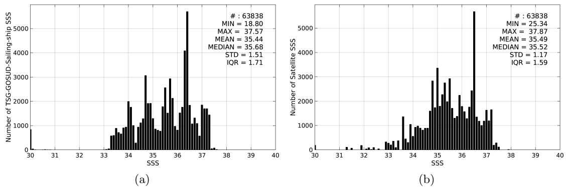
Figure 2: Histograms of SSS from TSG-GOSUD-Sailing-ship (a) and SMOS-L3-CATDS-CPDC-V3-10DAYS-25KM (b) considering all match-up pairs per bins of 0.1 over the South Atlantic Ocean Pi-MEP region and for the full satellite product period.
