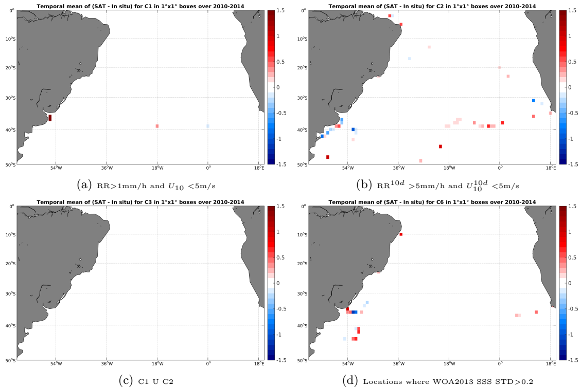
Figure 12: Temporal mean gridded over spatial boxes of size 1°x1° of \Delta SSS (SMOS-L3-CATDS-CPDC-V3-10DAYS-25KM - TSG-GOSUD-Sailing-ship) for 4 different subdatasets corresponding to: RR > 1mm/h and U_{10} < 5m/s (a), RR^{10d} > 5mm/h and U_{10}^{10d} < 5m/s (b), C1 U C2 (c), Locations where WOA2013 SSS STD > 0.2 (d).
