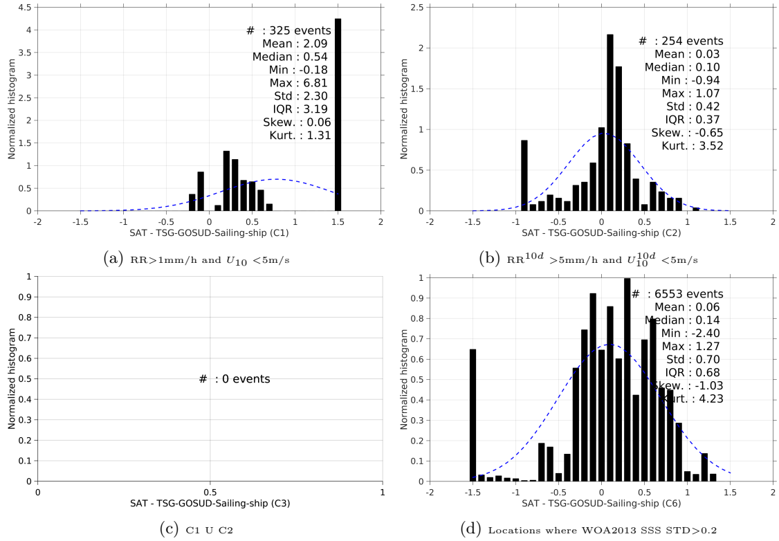
Figure 13: Normalized histogram of \Delta SSS (SMOS-L3-CATDS-CPDC-V3-10DAYS-25KM - TSG-GOSUD-Sailing-ship) for 6 different subdatasets corresponding to: RR > 1mm/h and U_{10} < 5\text{m/s} (a), RR^{10d} > 5\text{mm/h} and U_{10}^{10d} < 5\text{m/s} (b), C1 U C2 (c), Locations where WOA2013 SSS STD > 0.2 (d).
