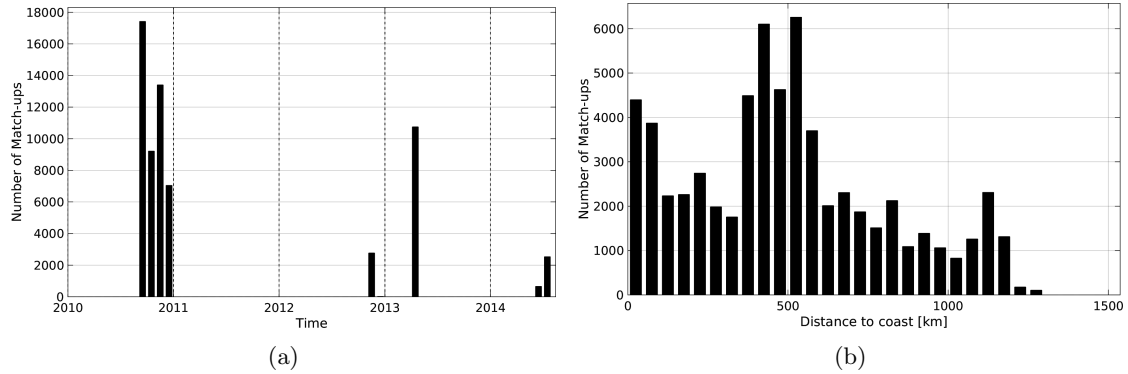
Figure 1: Number of match-ups between TSG-GOSUD-Sailing-ship and SMOS-L3-CATDS-CPDC-V3-10DAYS-25KM SSS as a function of time (a) and as function of the distance to coast (b) over the South Atlantic Ocean Pi-MEP region and for the full satellite product period.
