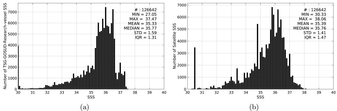
Figure 2: Histograms of SSS from TSG-GOSUD-Research-vessel (a) and SMOS-L3-CATDS-CPDC-V3-10DAYS-25KM (b) considering all match-up pairs per bins of 0.1 over the South Atlantic Ocean Pi-MEP region and for the full satellite product period.
