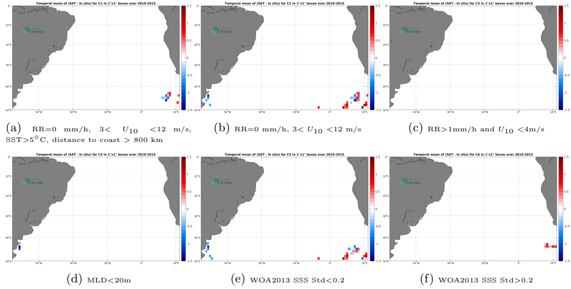
Figure 12: Temporal mean gridded over spatial boxes of size 1^\circ \times 1^\circ of \Delta SSS (SMOS-L3-CATDS-CPDC-V3-10DAYS-25KM - Sea mammals) for 6 different subdatasets corresponding to: RR=0 mm/h, 3 < U_{10} < 12 m/s, SST > 5^\circ C , distance to coast > 800 km (a), RR=0 mm/h, 3 < U_{10} < 12 m/s (b), RR > 1 mm/h and U_{10} < 4 m/s (c), MLD < 20 m (d), WOA2013 SSS Std < 0.2 (e), WOA2013 SSS Std > 0.2 (f).
