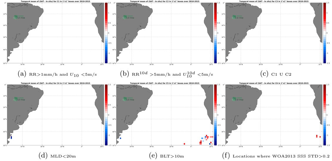
Figure 12: Temporal mean gridded over spatial boxes of size 1^\circ \times 1^\circ of \Delta\text{SSS} (SMOS-L3-CATDS-CPDC-V3-10DAYS-25KM - Sea mammals) for 6 different subdatasets corresponding to: RR > 1\text{mm/h} and U_{10} < 5\text{m/s} (a), RR^{10d} > 5\text{mm/h} and U_{10}^{10d} < 5\text{m/s} (b), C1 U C2 (c), MLD < 20\text{m} (d), BLT > 10\text{m} (e), Locations where WOA2013 SSS STD > 0.2 (f).
