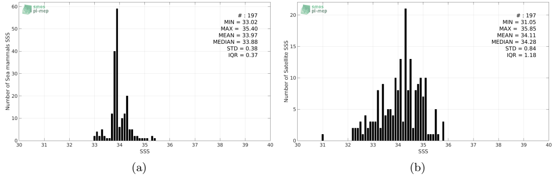
Figure 2: Histograms of SSS from Sea mammals (a) and SMOS-L3-CATDS-CPDC-V3-10DAYS-25KM (b) considering all match-up pairs per bins of 0.1 over the South Atlantic Ocean Pi-MEP region and for the full satellite product period.
