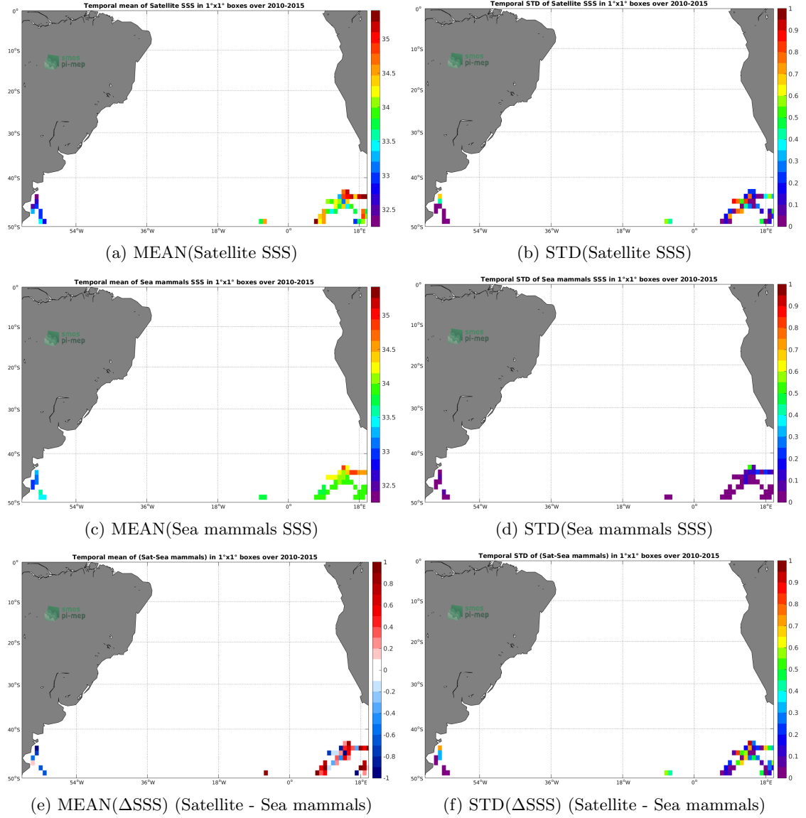
Figure 6: Temporal mean (left) and STD (right) of SSS from SMOS-L3-CATDS-CPDC-V3-10DAYS-25KM (top), Sea mammals (middle), and of \Delta SSS (Satellite - Sea mammals). Only match-up pairs are used to generate these maps.
