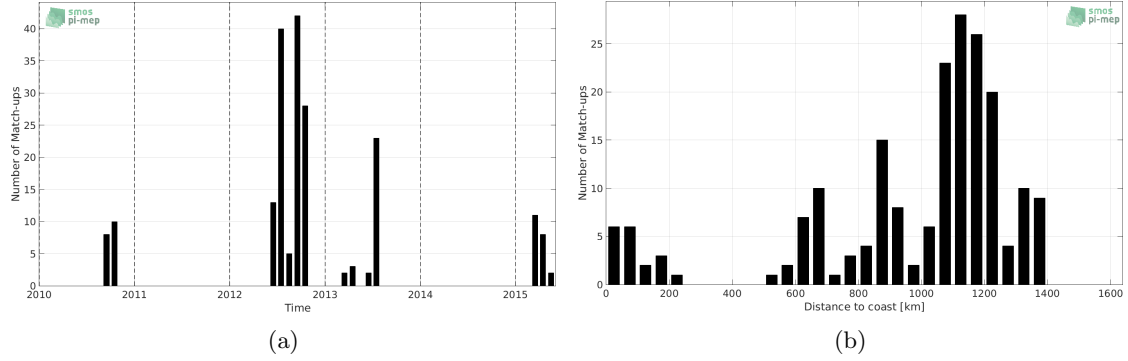
Figure 1: Number of match-ups between Sea mammals and SMOS-L3-CATDS-CPDC-V3-10DAYS-25KM SSS as a function of time (a) and as function of the distance to coast (b) over the South Atlantic Ocean Pi-MEP region and for the full satellite product period.
