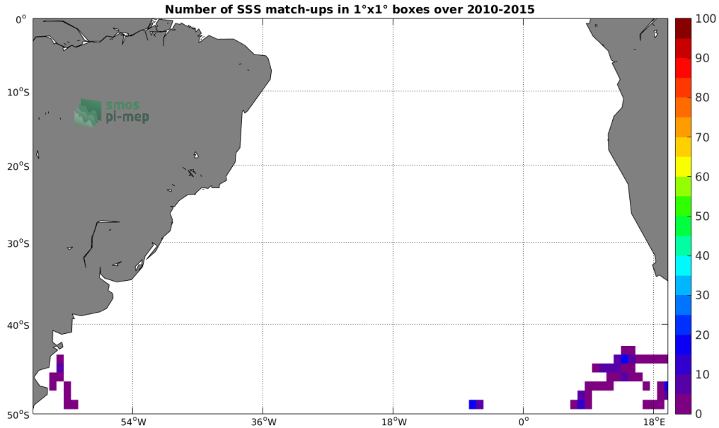
Figure 4: Number of SSS match-ups between Sea mammals SSS and the SMOS-L3-CATDS-CPDC-V3-10DAYS-25KM SSS product for the South Atlantic Ocean Pi-MEP region over 1^\circ \times 1^\circ boxes and for the full satellite product period.
