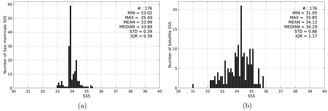
Figure 2: Histograms of SSS from Sea mammals (a) and SMOS-L3-CATDS-CPDC-V3-10DAYS-25KM (b) considering all match-up pairs per bins of 0.1 over the South Atlantic Ocean Pi-MEP region and for the full satellite product period.
