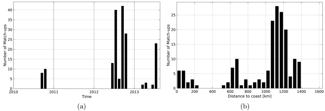
Figure 1: Number of match-ups between Sea mammals and SMOS-L3-CATDS-CPDC-V3-10DAYS-25KM SSS as a function of time (a) and as function of the distance to coast (b) over the South Atlantic Ocean Pi-MEP region and for the full satellite product period.
