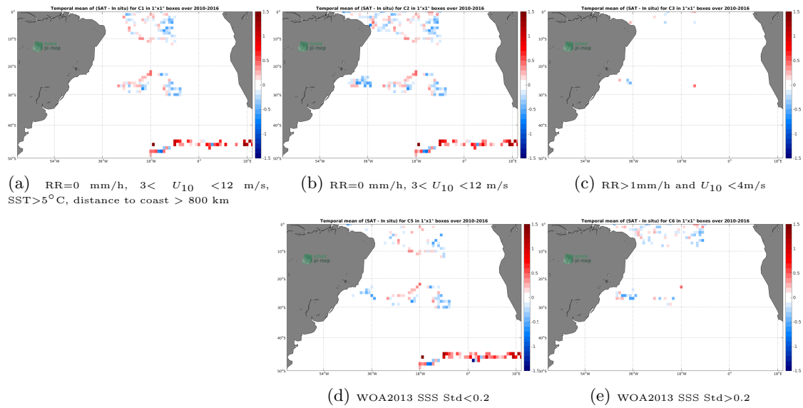
Figure 11: Temporal mean gridded over spatial boxes of size 1^\circ \times 1^\circ of \Delta SSS (SMOS-L3-CATDS-CPDC-V3-10DAYS-25KM - Surface drifters) for 5 different subdatasets corresponding to: RR=0 mm/h, 3 < U_{10} < 12 m/s, SST > 5^\circ C , distance to coast > 800 km (a), RR=0 mm/h, 3 < U_{10} < 12 m/s (b), RR > 1 mm/h and U_{10} < 4 m/s (c), WOA2013 SSS Std < 0.2 (d), WOA2013 SSS Std > 0.2 (e).
