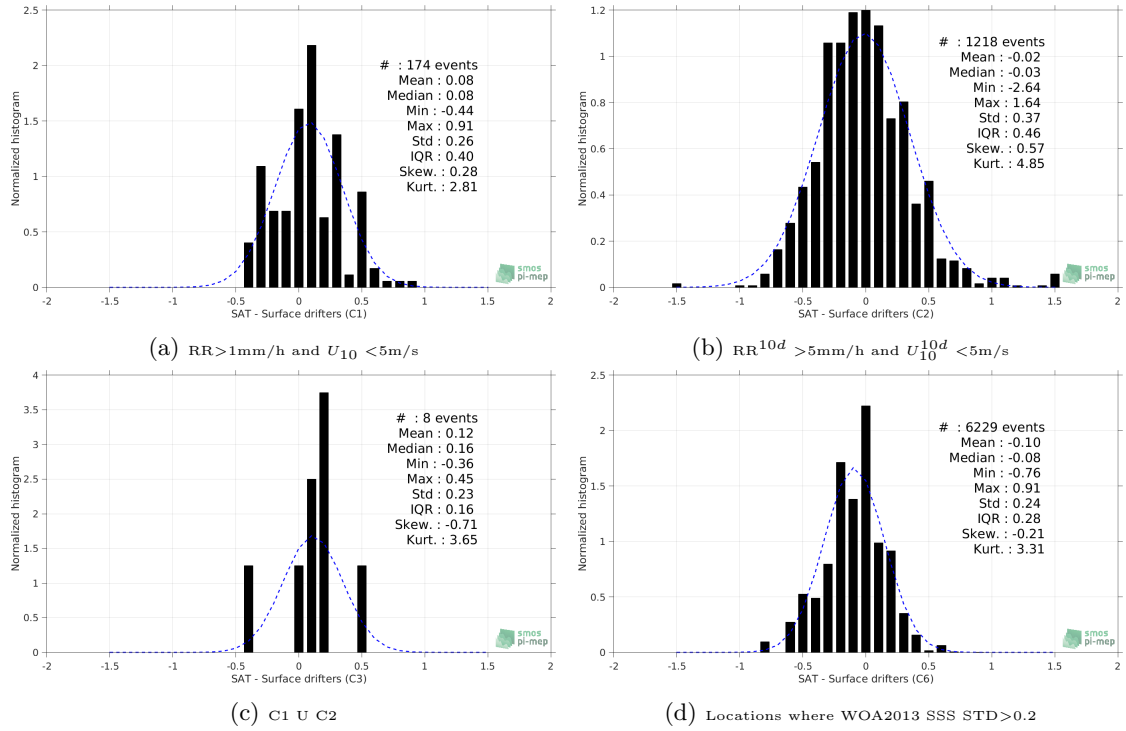
Figure 12: Normalized histogram of \Delta SSS (SMOS-L3-CATDS-CPDC-V3-10DAYS-25KM - Surface drifters) for 6 different subdatasets corresponding to: RR > 1mm/h and U_{10} < 5 m/s (a), RR^{10d} > 5 mm/h and U_{10}^{10d} < 5 m/s (b), C1 U C2 (c), Locations where WOA2013 SSS STD > 0.2 (d).
