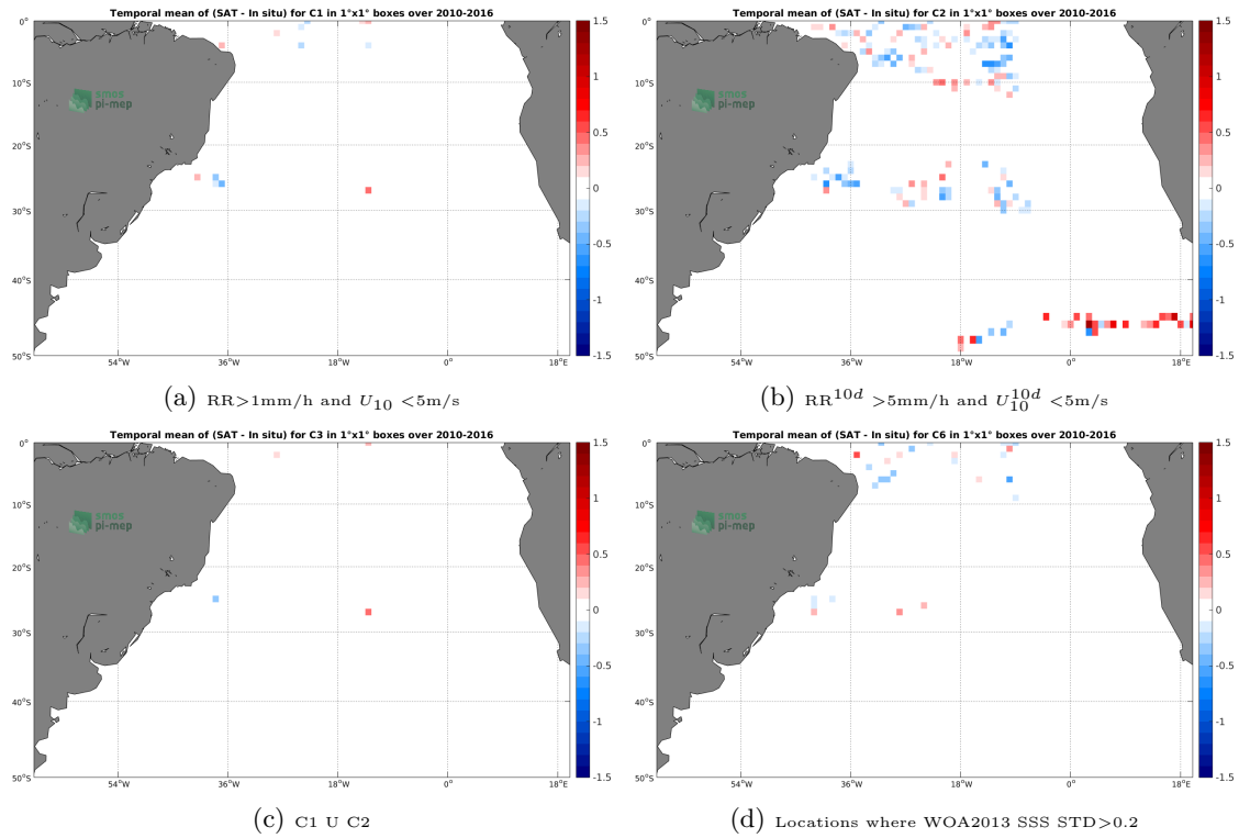
Figure 11: Temporal mean gridded over spatial boxes of size 1^\circ \times 1^\circ of \Delta SSS (SMOS-L3-CATDS-CPDC-V3-10DAYS-25KM - Surface drifters) for 4 different subdatasets corresponding to: RR > 1\text{mm/h} and U_{10} < 5\text{m/s} (a), RR^{10d} > 5\text{mm/h} and U_{10}^{10d} < 5\text{m/s} (b), C1 U C2 (c), Locations where WOA2013 SSS STD > 0.2 (d).
