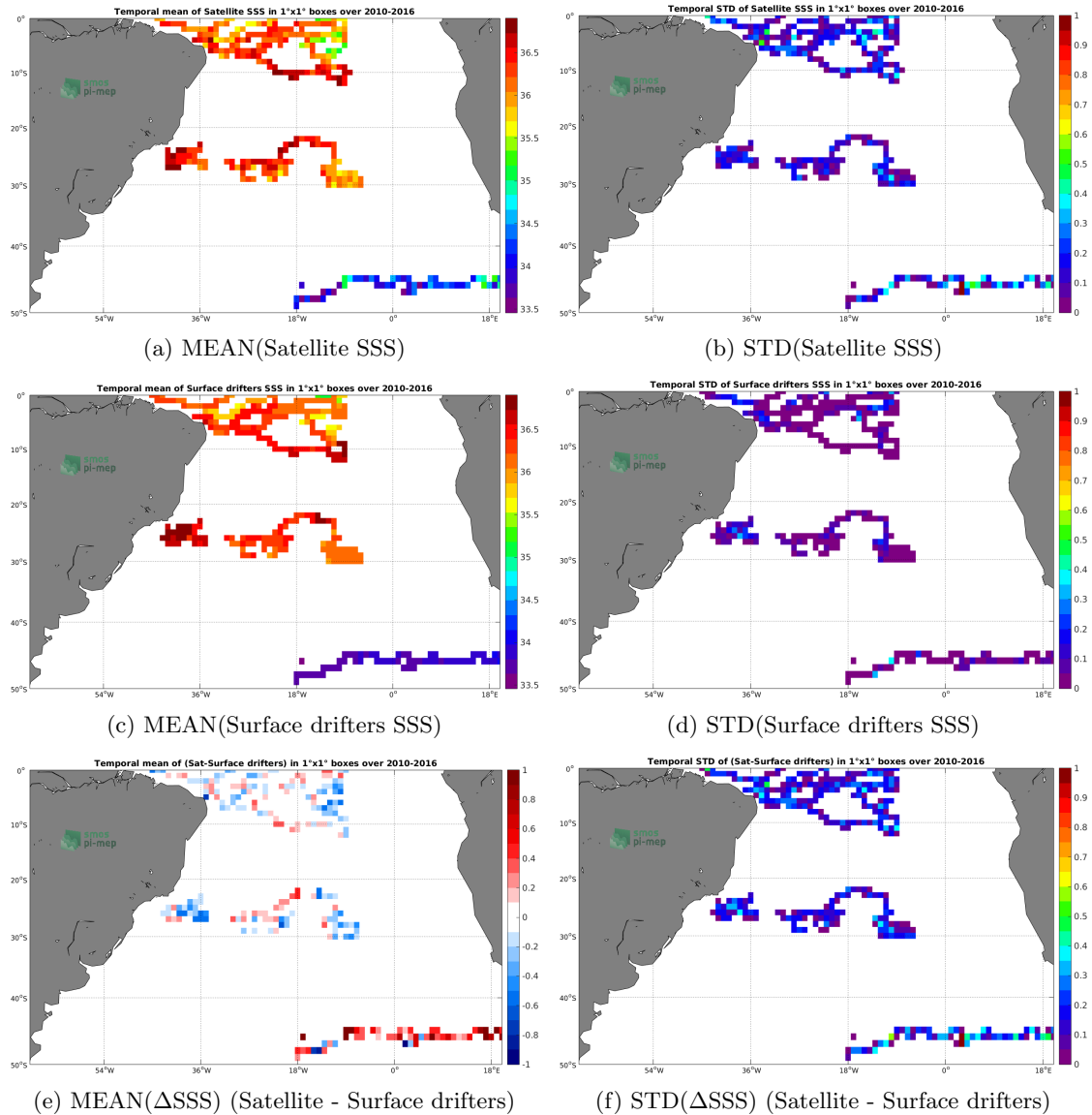
Figure 5: Temporal mean (left) and STD (right) of SSS from SMOS-L3-CATDS-CPDC-V3-10DAYS-25KM (top), Surface drifters (middle), and of \Delta SSS (Satellite - Surface drifters). Only match-up pairs are used to generate these maps.
