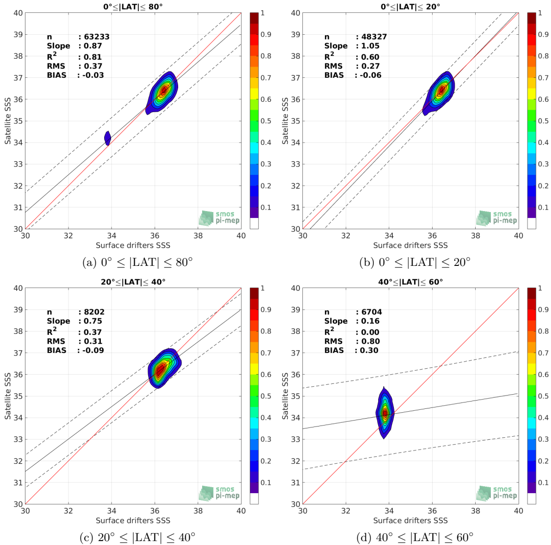
Figure 8: Contour maps of the concentration of SMOS-L3-CATDS-CPDC-V3-10DAYS-25KM SSS (y-axis) versus Surface drifters SSS (x-axis) at match-up pairs for different latitude bands. For each plot, the red line shows x=y . The black thin and dashed lines indicate a linear fit through the data cloud and the \pm 95\% confidence levels, respectively. The number match-up pairs n , the slope and R^2 coefficient of the linear fit, the root mean square (RMS) and the mean bias between satellite and in situ data are indicated for each latitude band in each plots.
