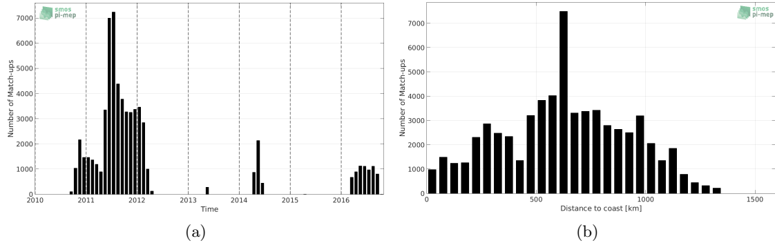
Figure 1: Number of match-ups between Surface drifters and SMOS-L3-CATDS-CPDC-V3-10DAYS-25KM SSS as a function of time (a) and as function of the distance to coast (b) over the South Atlantic Ocean Pi-MEP region and for the full satellite product period.
