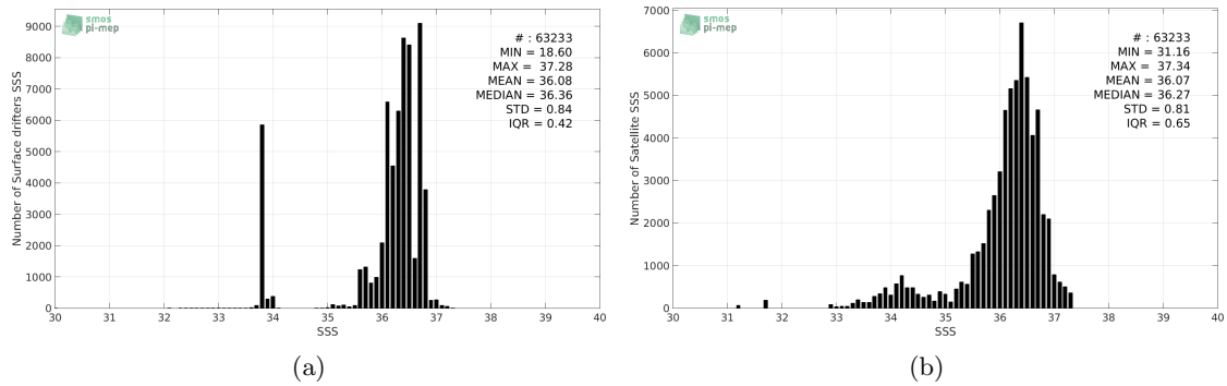
Figure 2: Histograms of SSS from Surface drifters (a) and SMOS-L3-CATDS-CPDC-V3-10DAYS-25KM (b) considering all match-up pairs per bins of 0.1 over the South Atlantic Ocean Pi-MEP region and for the full satellite product period.
