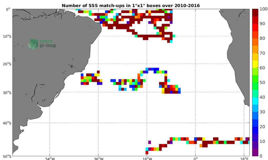
Figure 3: Number of SSS match-ups between Surface drifters SSS and the SMOS-L3-CATDS-CPDC-V3-10DAYS-25KM SSS product for the South Atlantic Ocean Pi-MEP region over 1^\circ \times 1^\circ boxes and for the full satellite product period.
