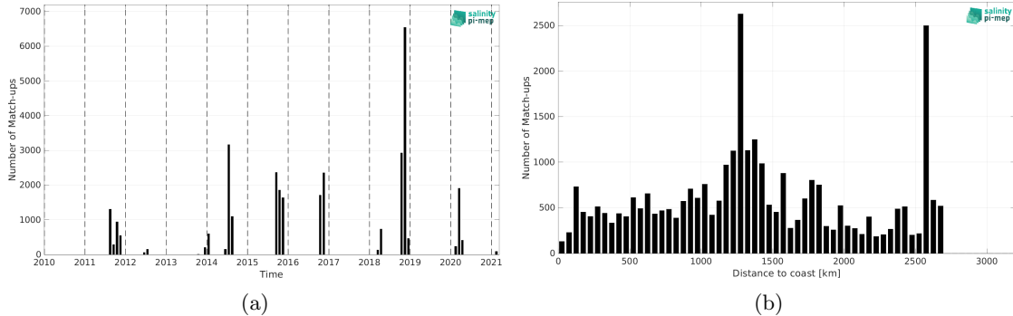
Figure 2: Number of match-ups between TSG (SAMOS) and SMOS SSS L3 v2 - 9-Days (BEC) SSS as a function of time (a) and as function of the distance to coast (b) over the South Atlantic Ocean Pi-MEP region and for the full satellite product period.
