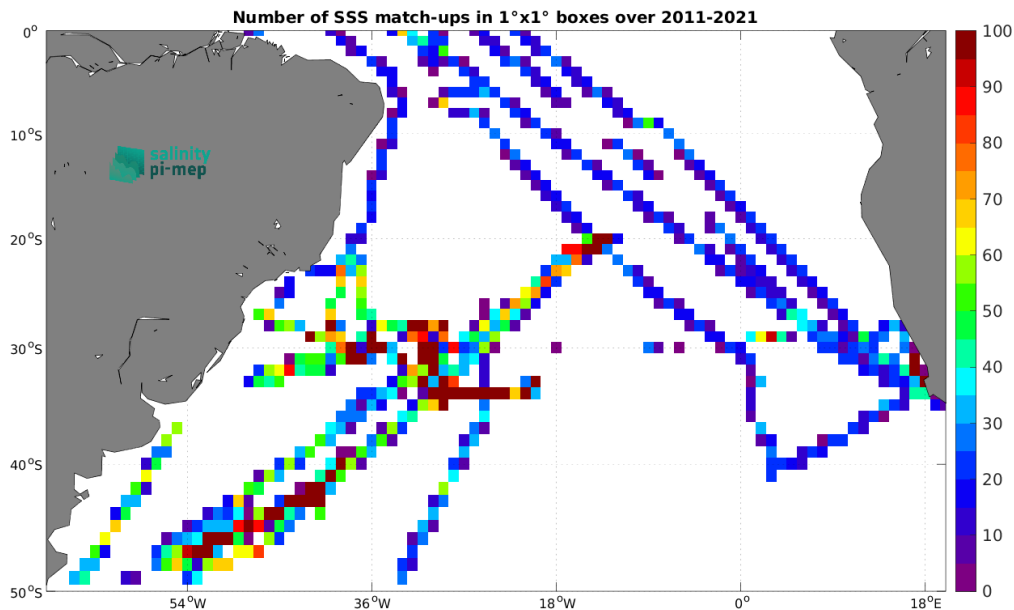
Figure 5: Number of SSS match-ups between TSG (SAMOS) SSS and the SMOS SSS L3 v2 - 9-Days (BEC) SSS product for the South Atlantic Ocean Pi-MEP region over 1^\circ \times 1^\circ boxes and for the full satellite product period.
