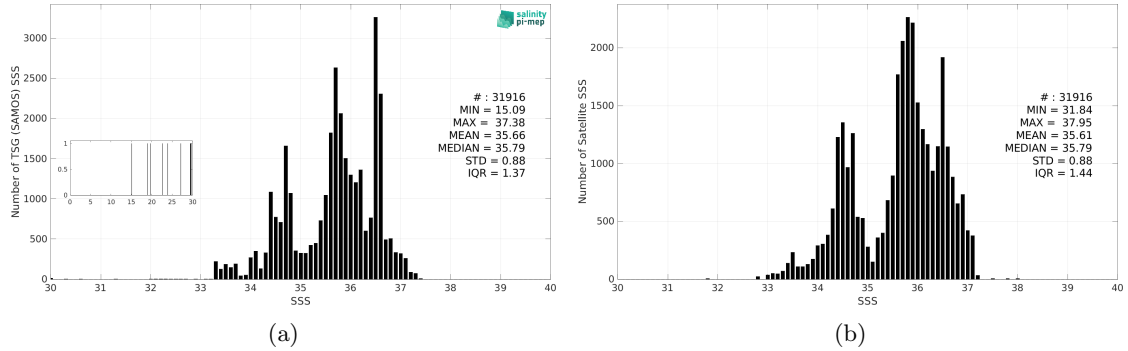
Figure 3: Histograms of SSS from TSG (SAMOS) (a) and SMOS SSS L3 v2 - 9-Days (BEC) (b) considering all match-up pairs per bins of 0.1 over the South Atlantic Ocean Pi-MEP region and for the full satellite product period.
