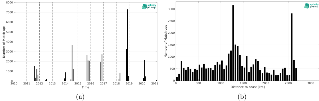
Figure 1: Number of match-ups between TSG (SAMOS) and SMOS SSS L3 v2 - 9-Days (BEC) SSS as a function of time (a) and as function of the distance to coast (b) over the South Atlantic Ocean Pi-MEP region and for the full satellite product period.
