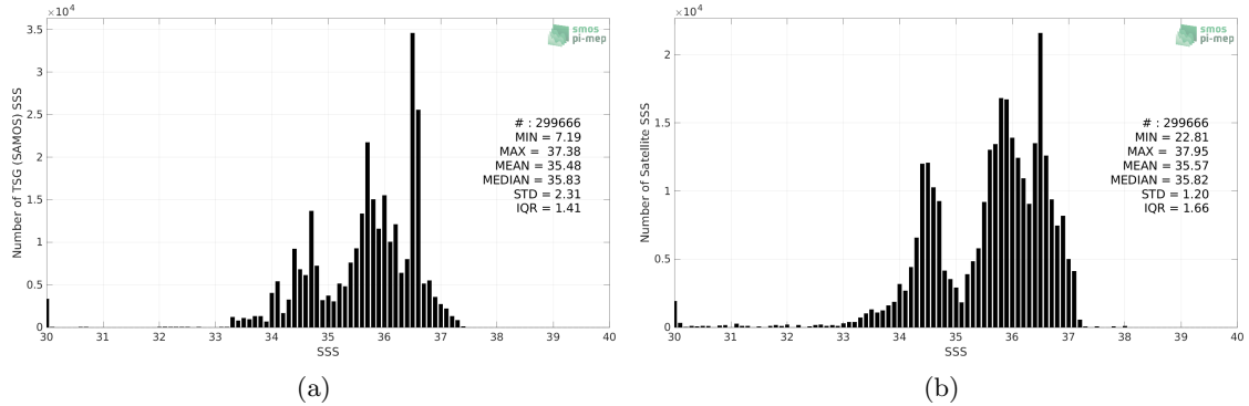
Figure 2: Histograms of SSS from TSG (SAMOS) (a) and SMOS SSS L3 v2 - 9-Days (BEC) (b) considering all match-up pairs per bins of 0.1 over the South Atlantic Ocean Pi-MEP region and for the full satellite product period.
