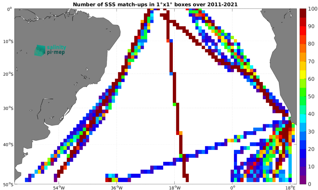
Figure 5: Number of SSS match-ups between TSG (Polarstern) SSS and the SMOS SSS L3 v2 - 9-Days (BEC) SSS product for the South Atlantic Ocean Pi-MEP region over 1^\circ \times 1^\circ boxes and for the full satellite product period.
