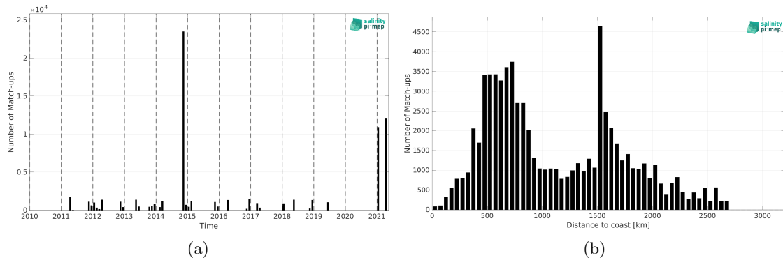
Figure 2: Number of match-ups between TSG (Polarstern) and SMOS SSS L3 v2 - 9-Days (BEC) SSS as a function of time (a) and as function of the distance to coast (b) over the South Atlantic Ocean Pi-MEP region and for the full satellite product period.
