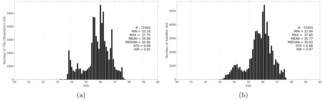
Figure 3: Histograms of SSS from TSG (Polarstern) (a) and SMOS SSS L3 v2 - 9-Days (BEC) (b) considering all match-up pairs per bins of 0.1 over the South Atlantic Ocean Pi-MEP region and for the full satellite product period.
