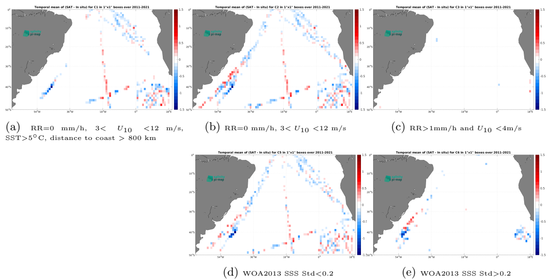
Figure 14: Temporal mean gridded over spatial boxes of size 1^\circ \times 1^\circ of \Delta SSS (SMOS SSS L3 v2 - 9-Days (BEC) - TSG (Polarstern)) for 5 different subdatasets corresponding to:RR=0 mm/h, 3 < U_{10} < 12 m/s, SST >5^\circ\text{C} , distance to coast > 800 km (a), RR=0 mm/h, 3 < U_{10} < 12 m/s (b), RR >1 mm/h and U_{10} < 4 m/s (c), WOA2013 SSS Std <0.2 (d), WOA2013 SSS Std >0.2 (e).
