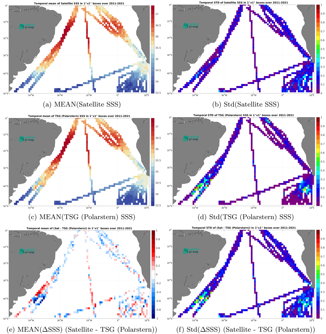
Figure 7: Temporal mean (left) and Std (right) of SSS from SMOS SSS L3 v2 - 9-Days (BEC) (top), TSG (Polarstern) (middle), and of \Delta SSS (Satellite - TSG (Polarstern)). Only match-up pairs are used to generate these maps.
