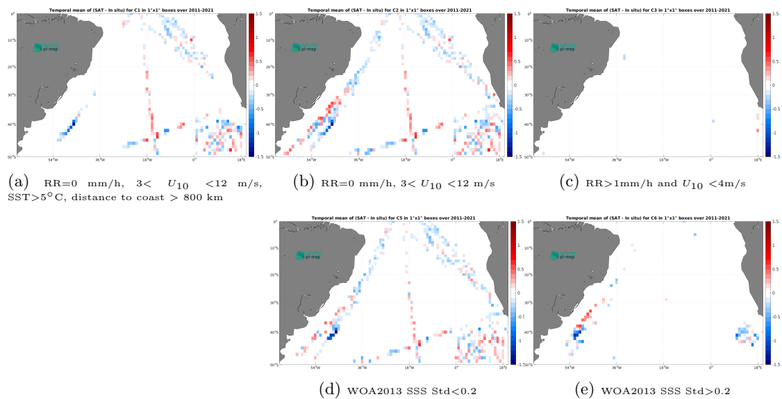
Figure 14: Temporal mean gridded over spatial boxes of size 1^\circ \times 1^\circ of \Delta SSS (SMOS SSS L3 v2 - 9-Days (BEC) - TSG (Polarstern)) for 5 different subdatasets corresponding to:RR=0 mm/h, 3 < U_{10} < 12 m/s, SST >5^\circ\text{C} , distance to coast > 800 km (a), RR=0 mm/h, 3 < U_{10} < 12 m/s (b), RR >1 mm/h and U_{10} < 4 m/s (c), WOA2013 SSS Std <0.2 (d), WOA2013 SSS Std >0.2 (e).
