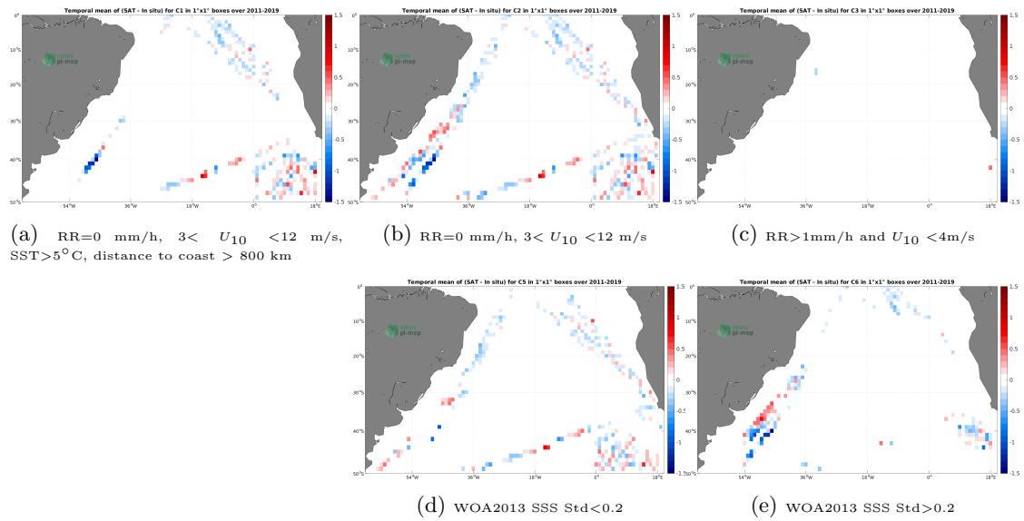
Figure 12: Temporal mean gridded over spatial boxes of size 1^\circ \times 1^\circ of \Delta\text{SSS} (SMOS SSS L3 v2 - 9-Days (BEC) - TSG (Polarstern)) for 5 different subdatasets corresponding to:RR=0 mm/h, 3 < U_{10} < 12 m/s, SST >5^\circ\text{C} , distance to coast > 800 km (a), RR=0 mm/h, 3 < U_{10} < 12 m/s (b), RR >1 mm/h and U_{10} < 4 m/s (c), WOA2013 SSS Std <0.2 (d), WOA2013 SSS Std >0.2 (e).
