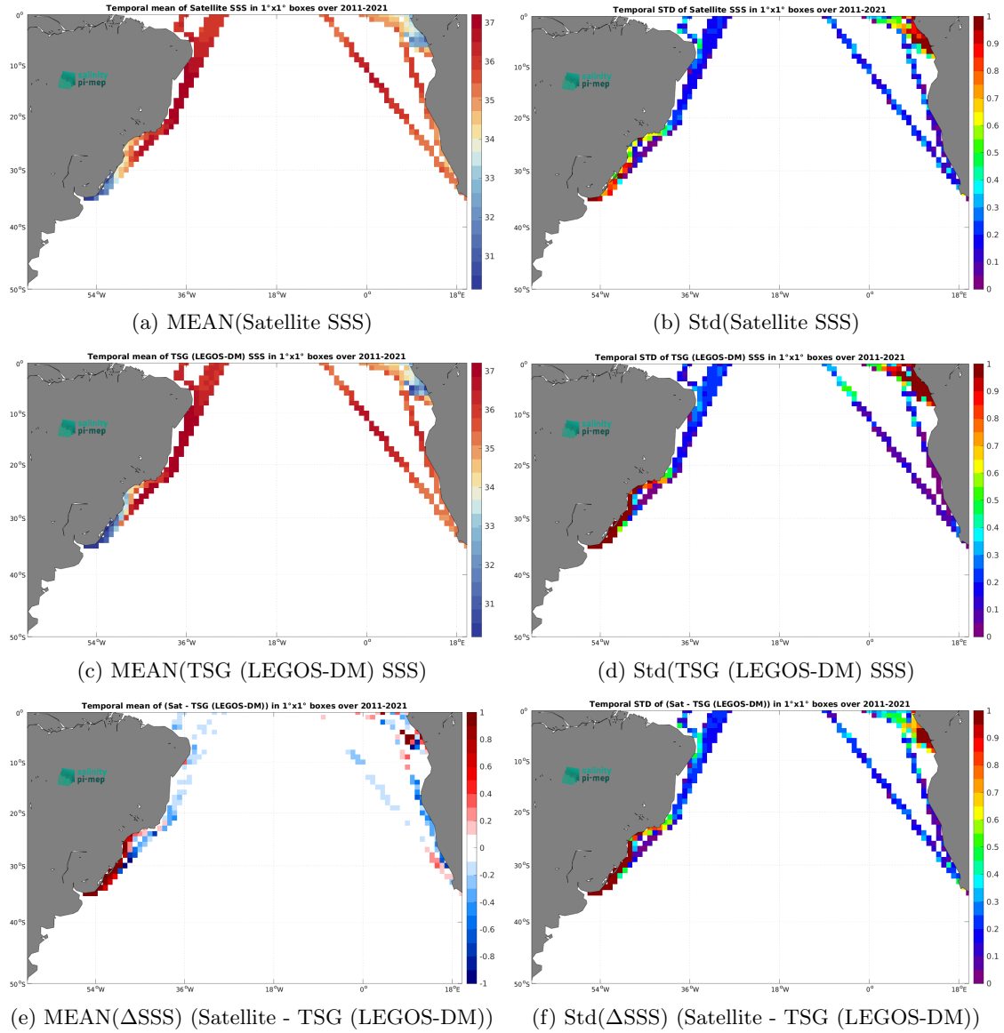
Figure 7: Temporal mean (left) and Std (right) of SSS from SMOS SSS L3 v2 - 9-Days (BEC) (top), TSG (LEGOS-DM) (middle), and of \Delta SSS (Satellite - TSG (LEGOS-DM)). Only match-up pairs are used to generate these maps.
