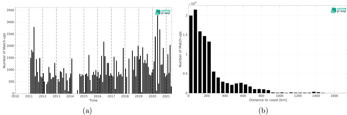
Figure 2: Number of match-ups between TSG (LEGOS-DM) and SMOS SSS L3 v2 - 9-Days (BEC) SSS as a function of time (a) and as function of the distance to coast (b) over the South Atlantic Ocean Pi-MEP region and for the full satellite product period.
