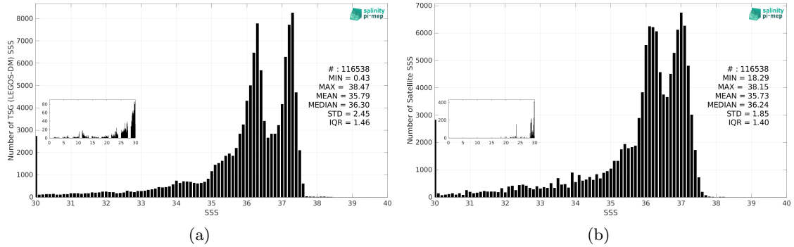
Figure 3: Histograms of SSS from TSG (LEGOS-DM) (a) and SMOS SSS L3 v2 - 9-Days (BEC) (b) considering all match-up pairs per bins of 0.1 over the South Atlantic Ocean Pi-MEP region and for the full satellite product period.
