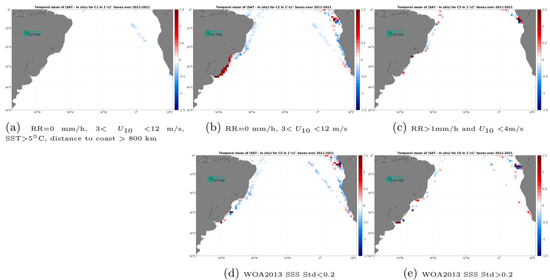
Figure 14: Temporal mean gridded over spatial boxes of size 1^\circ \times 1^\circ of \Delta\text{SSS} (SMOS SSS L3 v2 - 9-Days (BEC) - TSG (LEGOS-DM)) for 5 different subdatasets corresponding to:RR=0 mm/h, 3 < U_{10} < 12 m/s, SST >5^\circ\text{C} , distance to coast > 800 km (a), RR=0 mm/h, 3 < U_{10} < 12 m/s (b), RR >1 mm/h and U_{10} < 4 m/s (c), WOA2013 SSS Std <0.2 (d), WOA2013 SSS Std >0.2 (e).
