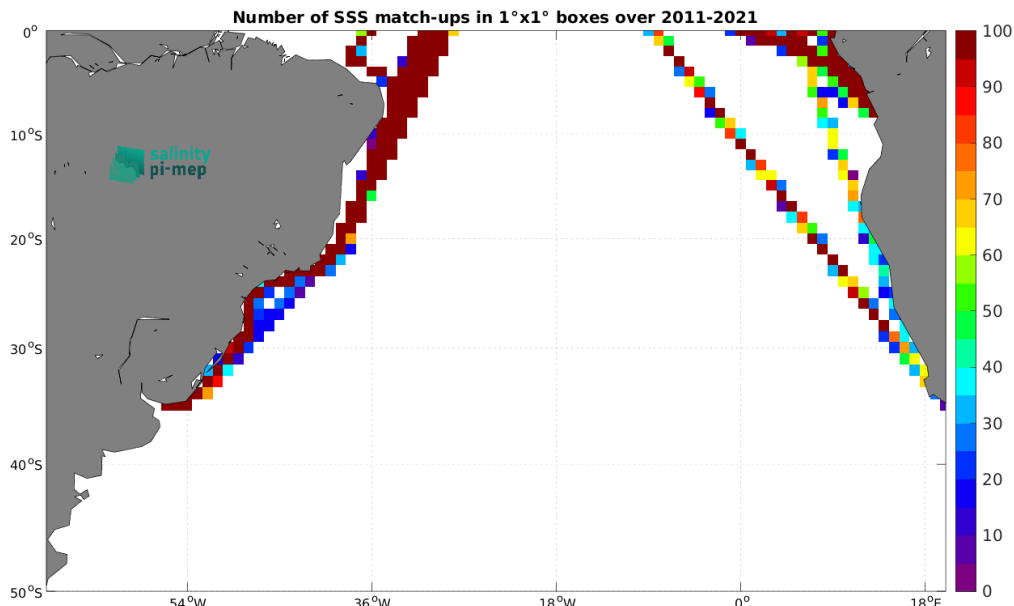
Figure 5: Number of SSS match-ups between TSG (LEGOS-DM) SSS and the SMOS SSS L3 v2 - 9-Days (BEC) SSS product for the South Atlantic Ocean Pi-MEP region over 1^\circ \times 1^\circ boxes and for the full satellite product period.
