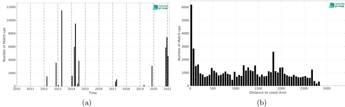
Figure 2: Number of match-ups between TSG (GOSUD-Sailing-ship) and SMOS SSS L3 v2 - 9-Days (BEC) SSS as a function of time (a) and as function of the distance to coast (b) over the South Atlantic Ocean Pi-MEP region and for the full satellite product period.
