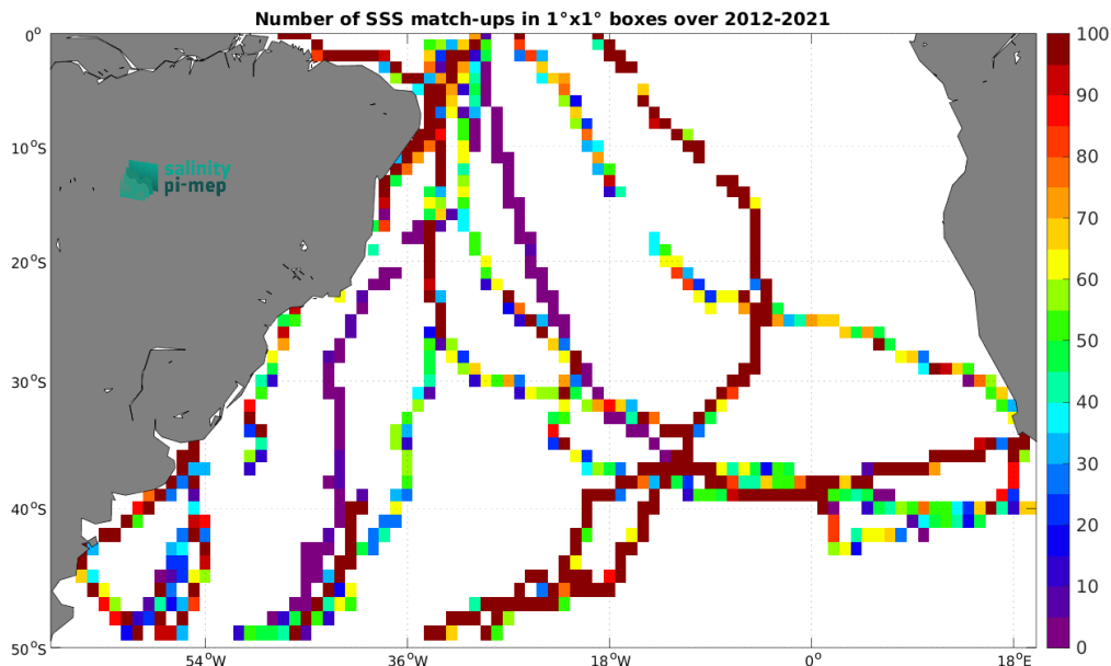
Figure 5: Number of SSS match-ups between TSG (GOSUD-Sailing-ship) SSS and the SMOS SSS L3 v2 - 9-Days (BEC) SSS product for the South Atlantic Ocean Pi-MEP region over 1^\circ \times 1^\circ boxes and for the full satellite product period.
