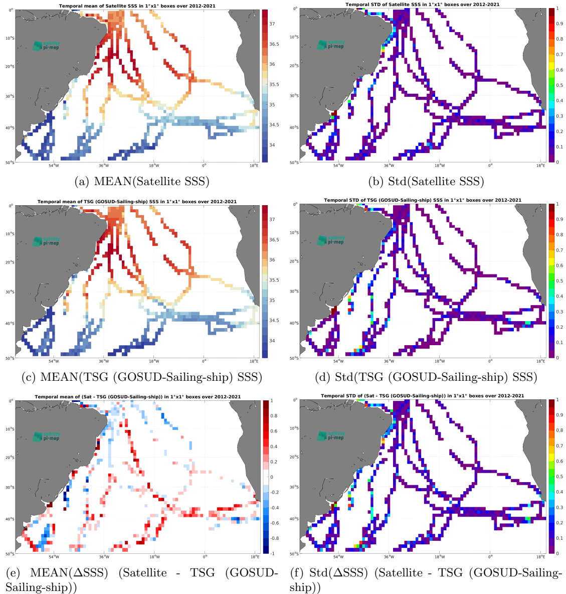
Figure 7: Temporal mean (left) and Std (right) of SSS from SMOS SSS L3 v2 - 9-Days (BEC) (top), TSG (GOSUD-Sailing-ship) (middle), and of \Delta SSS (Satellite - TSG (GOSUD-Sailing-ship)). Only match-up pairs are used to generate these maps.
