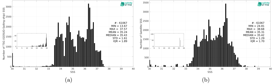
Figure 3: Histograms of SSS from TSG (GOSUD-Sailing-ship) (a) and SMOS SSS L3 v2 - 9-Days (BEC) (b) considering all match-up pairs per bins of 0.1 over the South Atlantic Ocean Pi-MEP region and for the full satellite product period.
