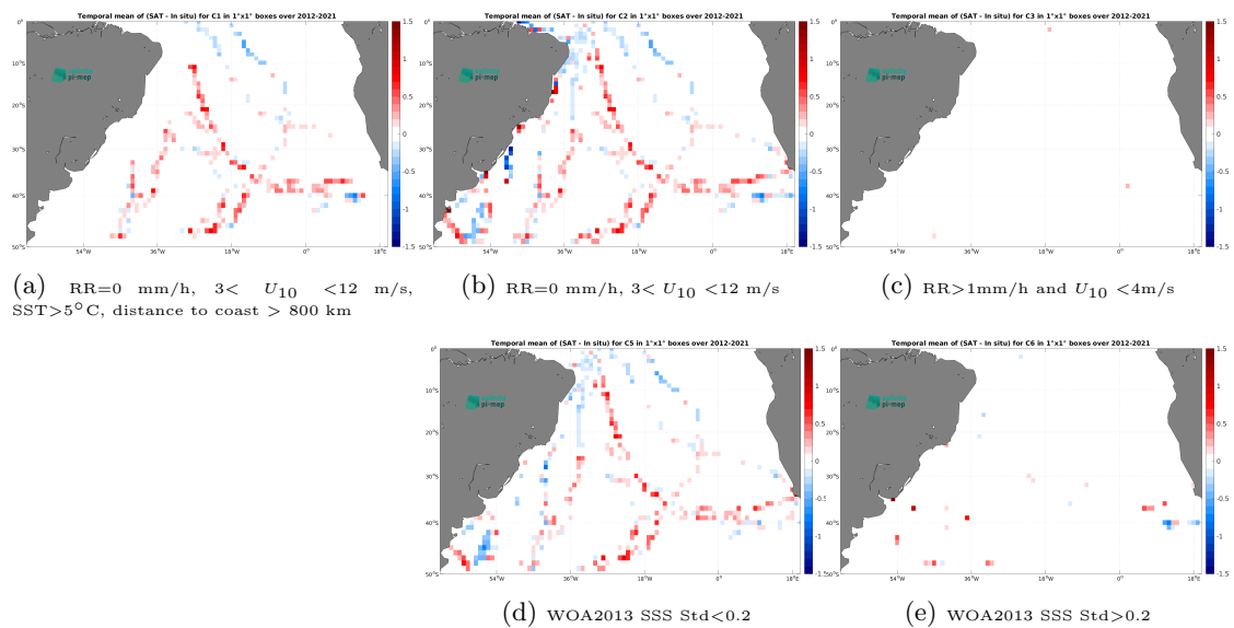
Figure 14: Temporal mean gridded over spatial boxes of size 1^\circ \times 1^\circ of \Delta\text{SSS} (SMOS SSS L3 v2 - 9-Days (BEC) - TSG (GOSUD-Sailing-ship)) for 5 different subdatasets corresponding to:RR=0 mm/h, 3 < U_{10} < 12 m/s, SST >5^\circ\text{C} , distance to coast > 800 km (a), RR=0 mm/h, 3 < U_{10} < 12 m/s (b), RR >1 mm/h and U_{10} < 4 m/s (c), WOA2013 SSS Std <0.2 (d), WOA2013 SSS Std >0.2 (e).
