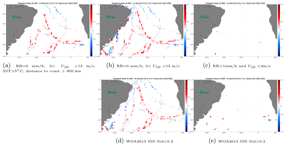
Figure 12: Temporal mean gridded over spatial boxes of size 1^\circ \times 1^\circ of \Delta\text{SSS} (SMOS SSS L3 v2 - 9-Days (BEC) - TSG (GOSUD-Sailing-ship)) for 5 different subdatasets corresponding to:RR=0 mm/h, 3 < U_{10} < 12 m/s, SST >5^\circ\text{C} , distance to coast > 800 km (a), RR=0 mm/h, 3 < U_{10} < 12 m/s (b), RR >1 mm/h and U_{10} < 4 m/s (c), WOA2013 SSS Std <0.2 (d), WOA2013 SSS Std >0.2 (e).
