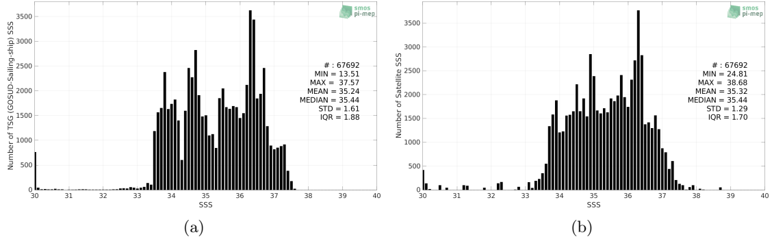
Figure 2: Histograms of SSS from TSG (GOSUD-Sailing-ship) (a) and SMOS SSS L3 v2 - 9-Days (BEC) (b) considering all match-up pairs per bins of 0.1 over the South Atlantic Ocean Pi-MEP region and for the full satellite product period.
