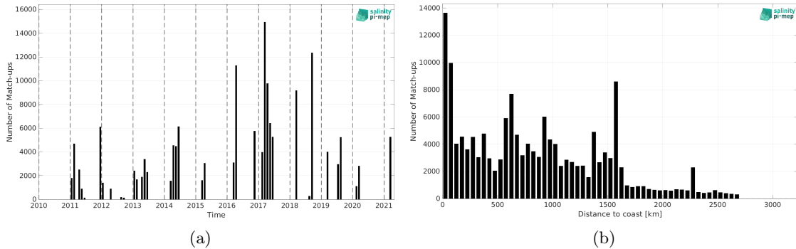
Figure 2: Number of match-ups between TSG (GOSUD-Research-vessel) and SMOS SSS L3 v2 - 9-Days (BEC) SSS as a function of time (a) and as function of the distance to coast (b) over the South Atlantic Ocean Pi-MEP region and for the full satellite product period.
