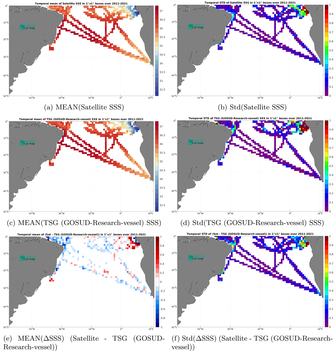
Figure 7: Temporal mean (left) and Std (right) of SSS from SMOS SSS L3 v2 - 9-Days (BEC) (top), TSG (GOSUD-Research-vessel) (middle), and of \Delta SSS (Satellite - TSG (GOSUD-Research-vessel)). Only match-up pairs are used to generate these maps.
