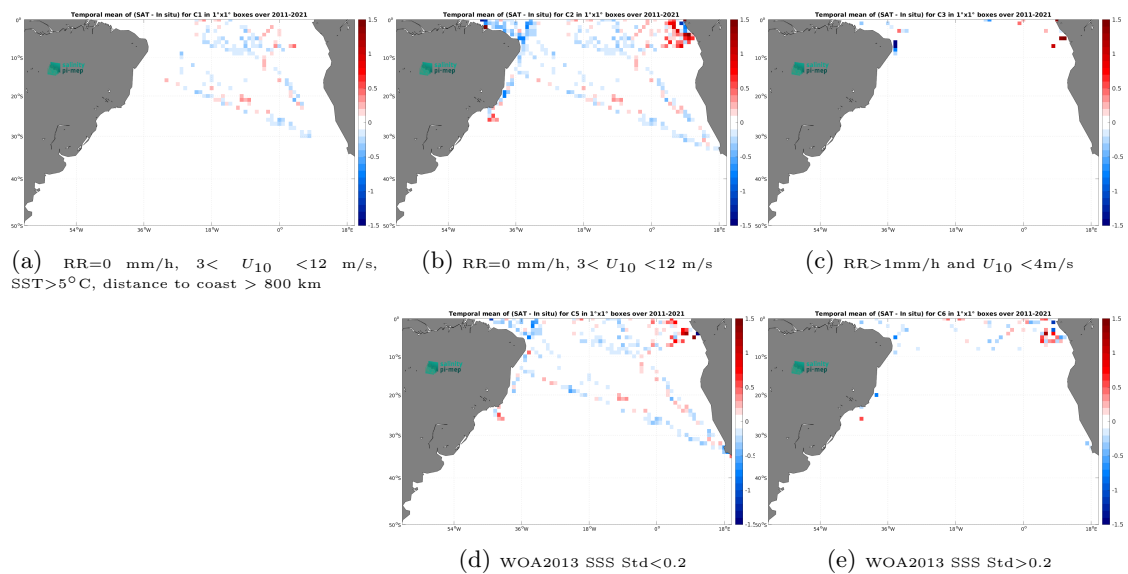
Figure 14: Temporal mean gridded over spatial boxes of size 1^\circ \times 1^\circ of \Delta SSS (SMOS SSS L3 v2 - 9-Days (BEC) - TSG (GOSUD-Research-vessel)) for 5 different subdatasets corresponding to:RR=0 mm/h, 3 < U_{10} < 12 m/s, SST >5^\circ\text{C} , distance to coast > 800 km (a), RR=0 mm/h, 3 < U_{10} < 12 m/s (b), RR >1 mm/h and U_{10} < 4 m/s (c), WOA2013 SSS Std <0.2 (d), WOA2013 SSS Std >0.2 (e).
