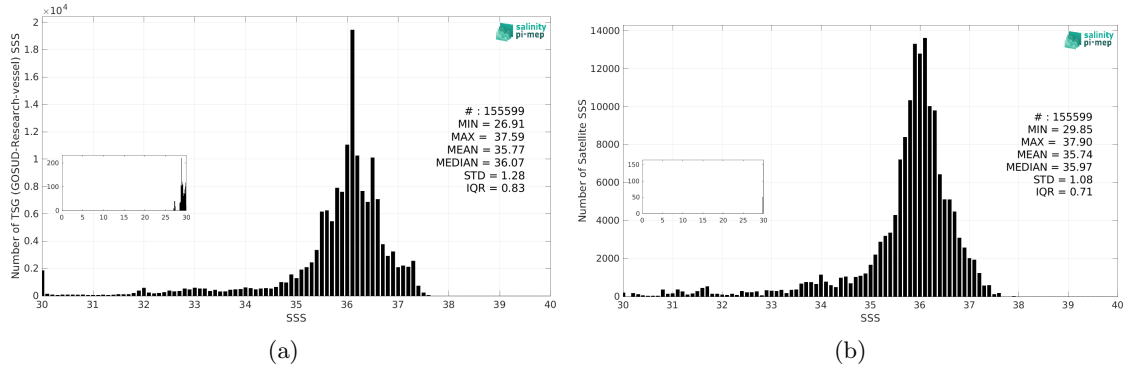
Figure 3: Histograms of SSS from TSG (GOSUD-Research-vessel) (a) and SMOS SSS L3 v2 - 9-Days (BEC) (b) considering all match-up pairs per bins of 0.1 over the South Atlantic Ocean Pi-MEP region and for the full satellite product period.
