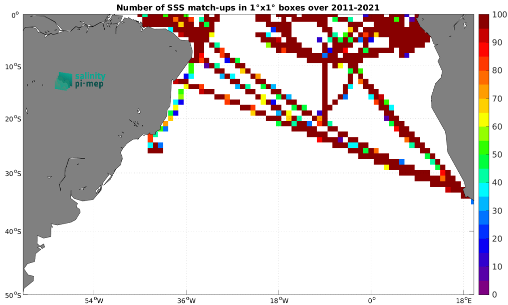
Figure 5: Number of SSS match-ups between TSG (GOSUD-Research-vessel) SSS and the SMOS SSS L3 v2 - 9-Days (BEC) SSS product for the South Atlantic Ocean Pi-MEP region over 1^{\circ} \times 1^{\circ} boxes and for the full satellite product period.
