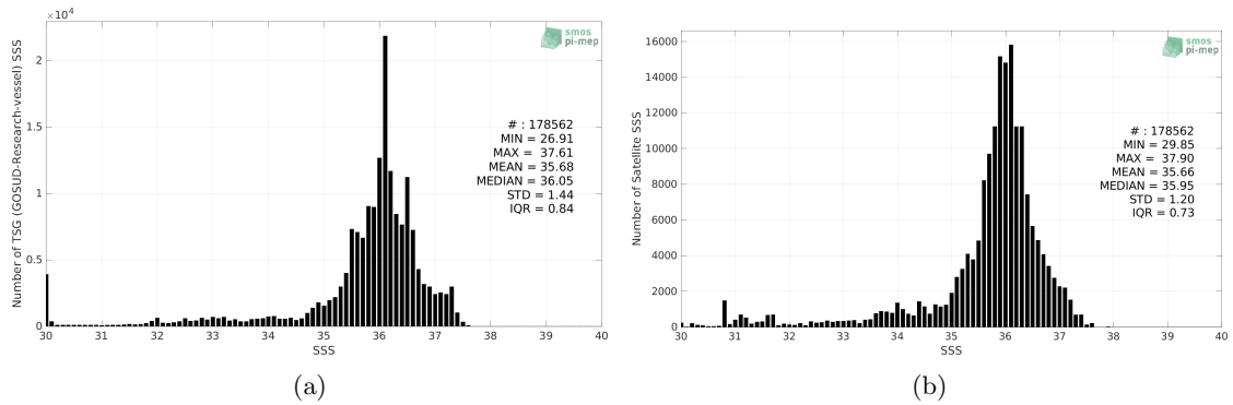
Figure 2: Histograms of SSS from TSG (GOSUD-Research-vessel) (a) and SMOS SSS L3 v2 - 9-Days (BEC) (b) considering all match-up pairs per bins of 0.1 over the South Atlantic Ocean Pi-MEP region and for the full satellite product period.
