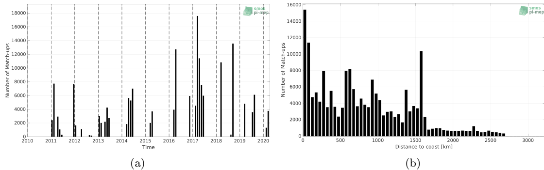
Figure 1: Number of match-ups between TSG (GOSUD-Research-vessel) and SMOS SSS L3 v2 - 9-Days (BEC) SSS as a function of time (a) and as function of the distance to coast (b) over the South Atlantic Ocean Pi-MEP region and for the full satellite product period.
