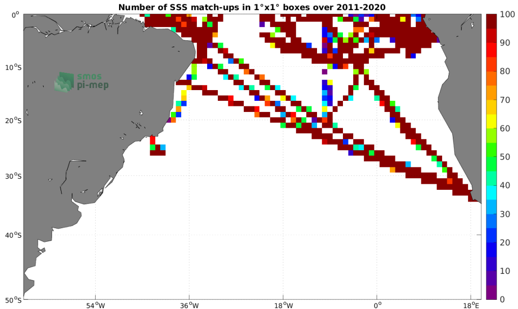
Figure 4: Number of SSS match-ups between TSG (GOSUD-Research-vessel) SSS and the SMOS SSS L3 v2 - 9-Days (BEC) SSS product for the South Atlantic Ocean Pi-MEP region over 1^\circ \times 1^\circ boxes and for the full satellite product period.
