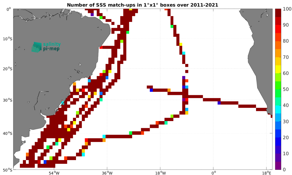
Figure 5: Number of SSS match-ups between TSG (CSIC-UTM) SSS and the SMOS SSS L3 v2 - 9-Days (BEC) SSS product for the South Atlantic Ocean Pi-MEP region over 1^\circ \times 1^\circ boxes and for the full satellite product period.
