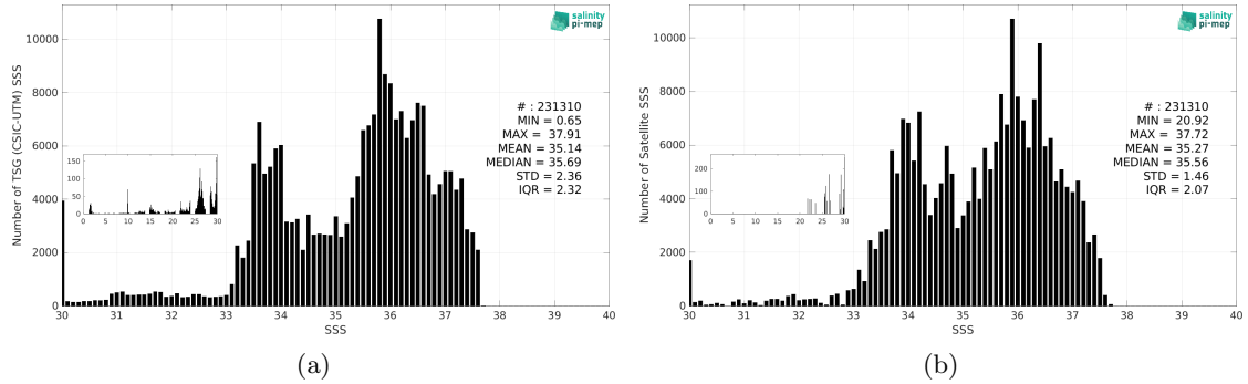
Figure 3: Histograms of SSS from TSG (CSIC-UTM) (a) and SMOS SSS L3 v2 - 9-Days (BEC) (b) considering all match-up pairs per bins of 0.1 over the South Atlantic Ocean Pi-MEP region and for the full satellite product period.
