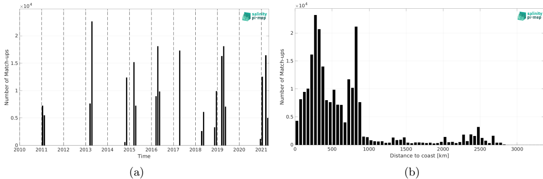
Figure 2: Number of match-ups between TSG (CSIC-UTM) and SMOS SSS L3 v2 - 9-Days (BEC) SSS as a function of time (a) and as function of the distance to coast (b) over the South Atlantic Ocean Pi-MEP region and for the full satellite product period.
